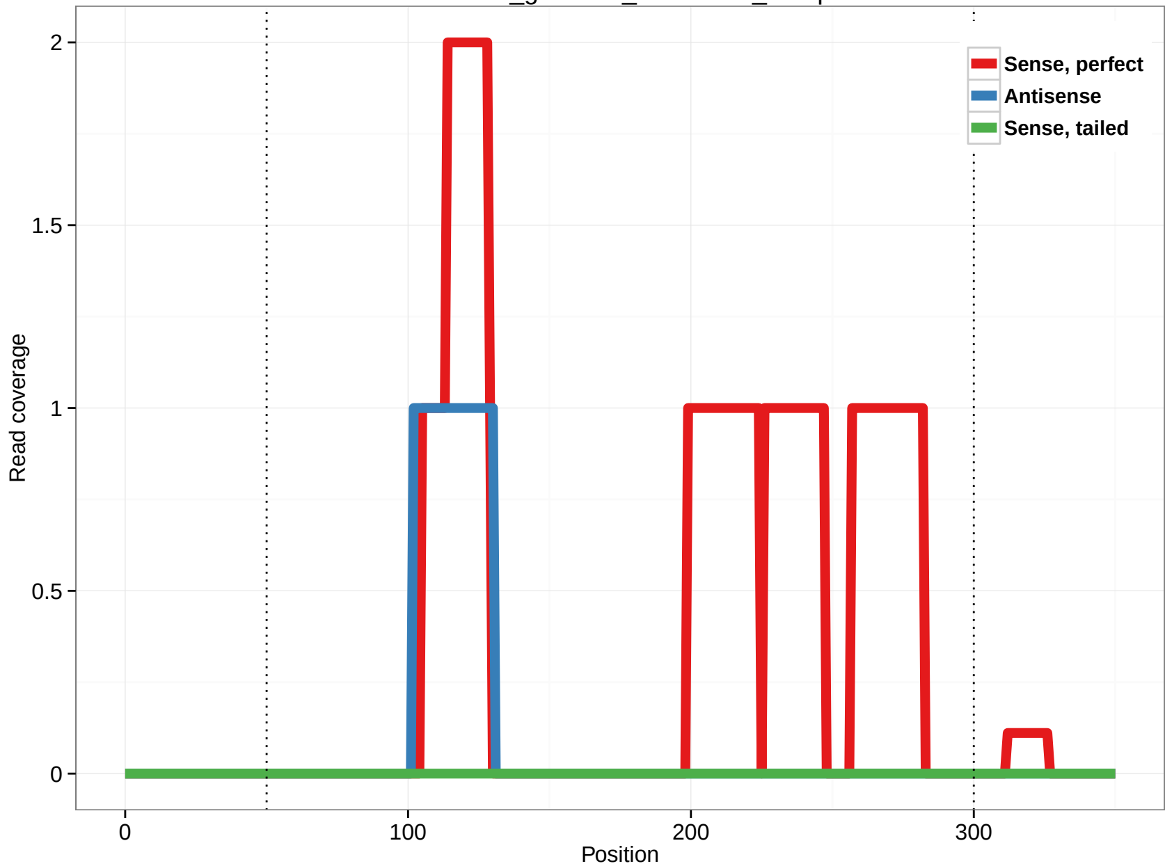
rheMac3_genscan_chr7.3057_17.3p
