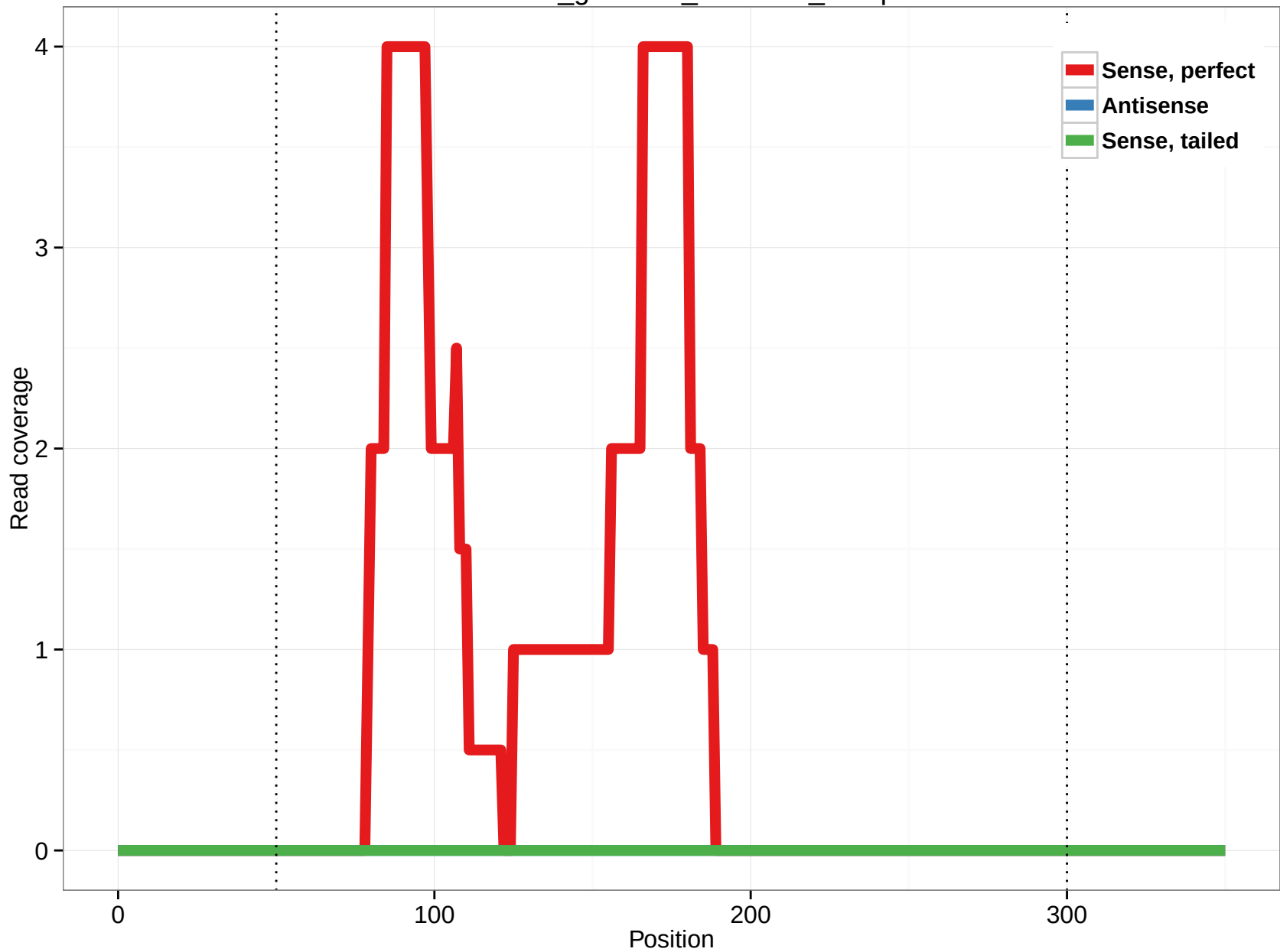
rheMac3_genscan_chr7.304_18.3p
