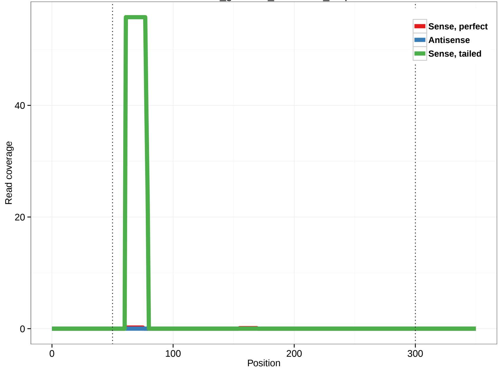
rheMac3_genscan_chr7.3004_4.5p
