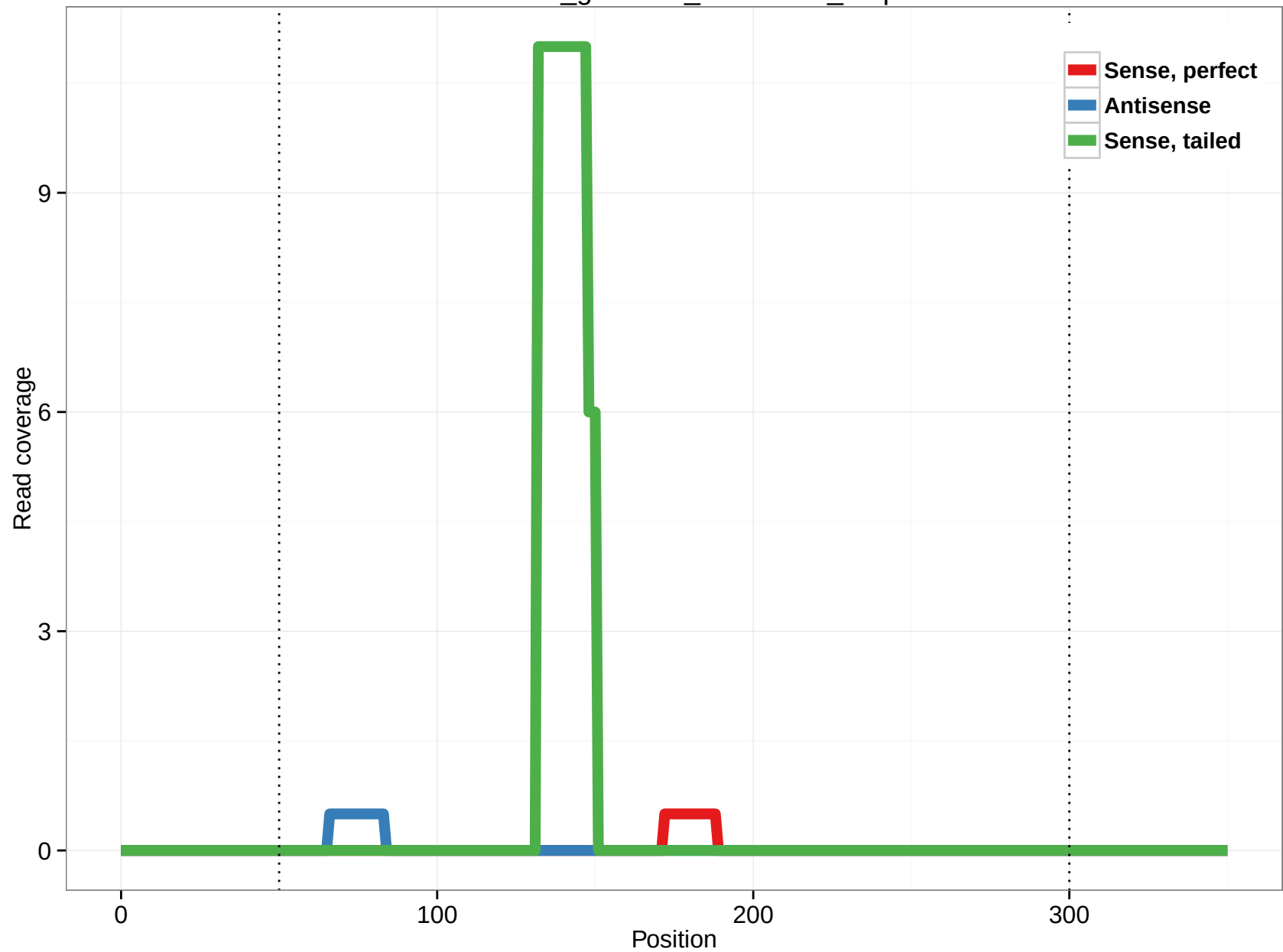
rheMac3_genscan_chr7.3001_4.3p
