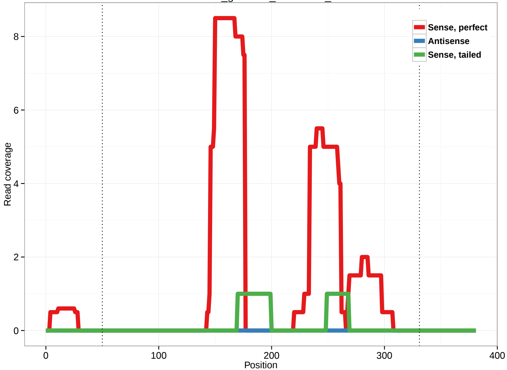
rheMac3_genscan_chr7.2977_11
