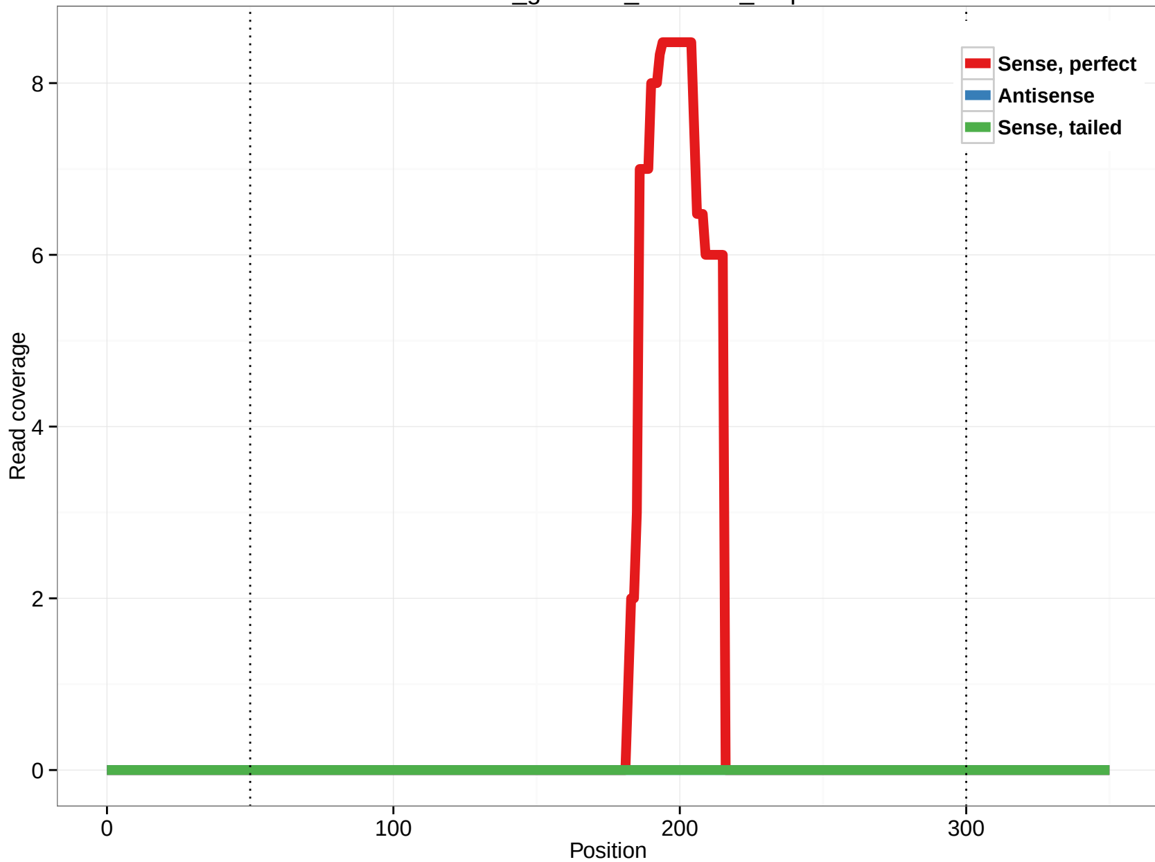
rheMac3_genscan_chr7.275_9.5p
