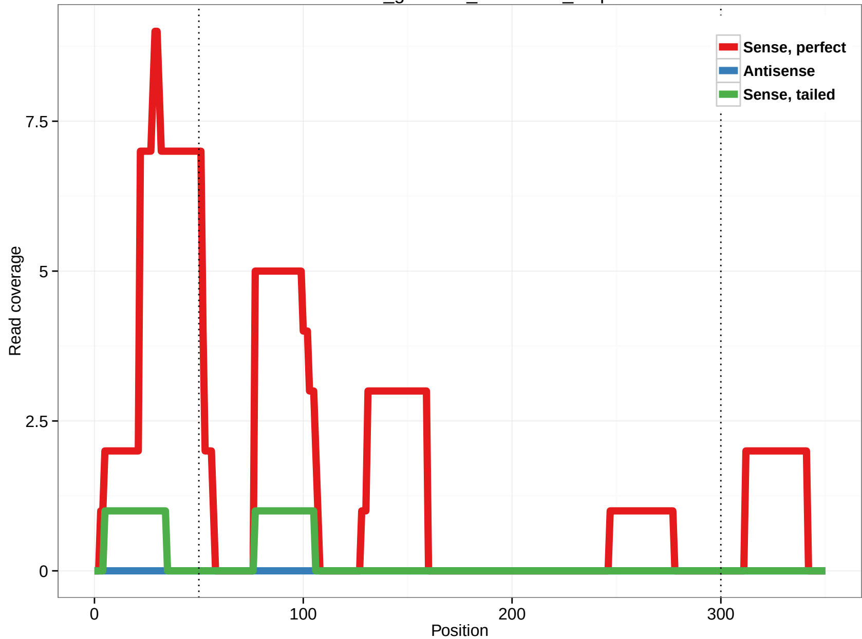
rheMac3_genscan_chr7.2735_9.3p
