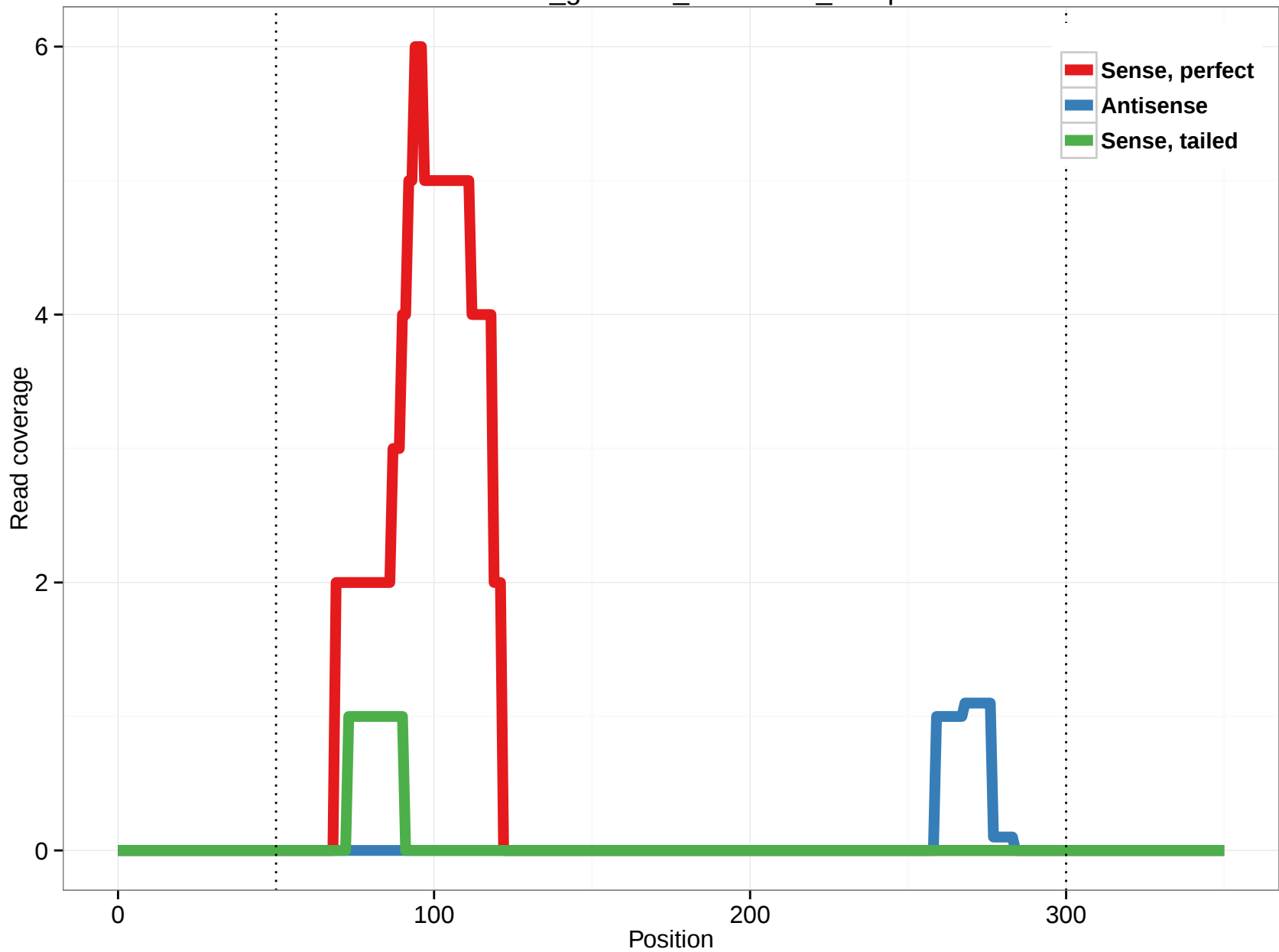
rheMac3_genscan_chr7.2703_14.5p
