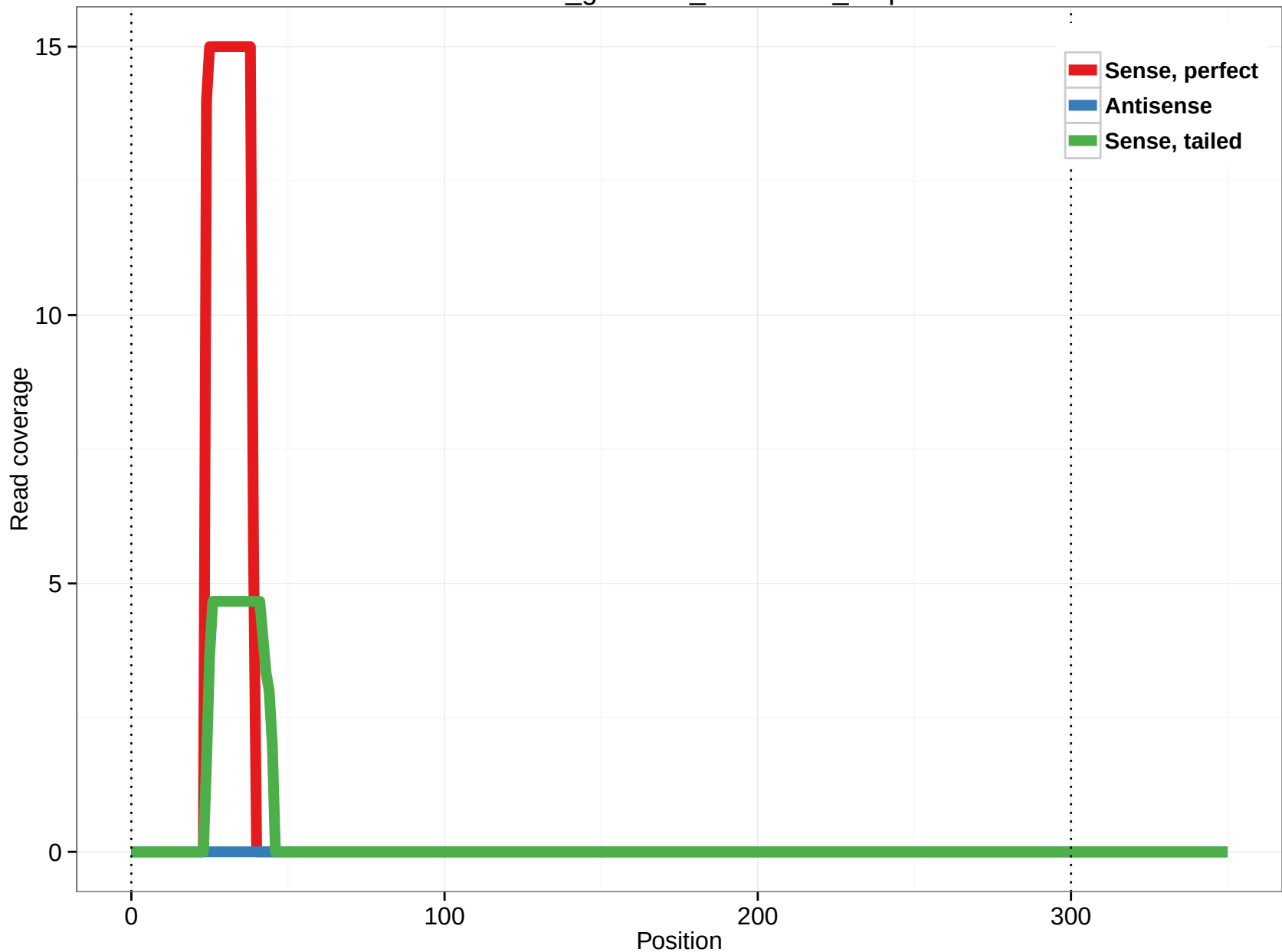
rheMac3_genscan_chr7.2693_2.3p
