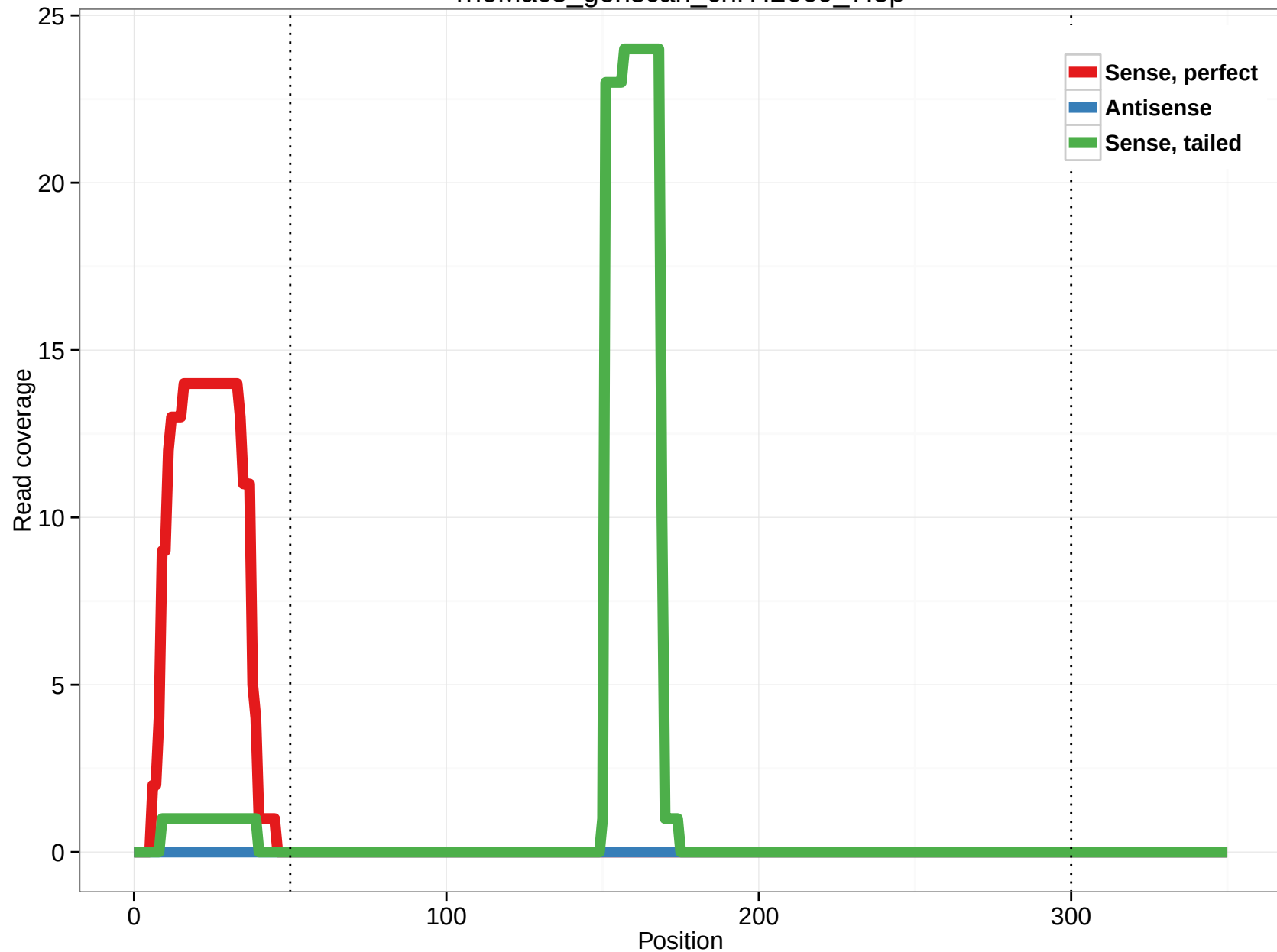
rheMac3_genscan_chr7.2669_7.5p
