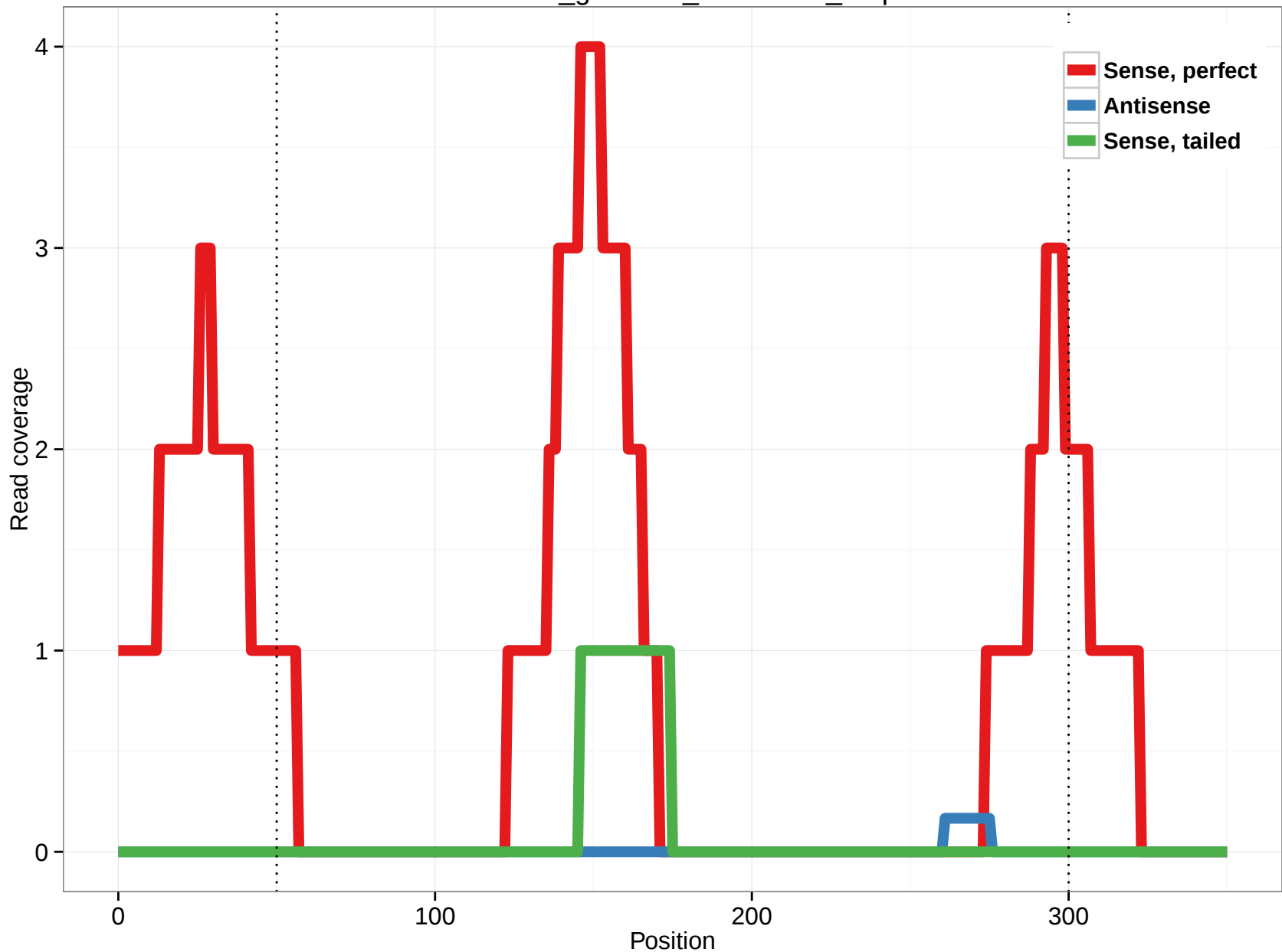
rheMac3_genscan_chr7.2659_9.5p
