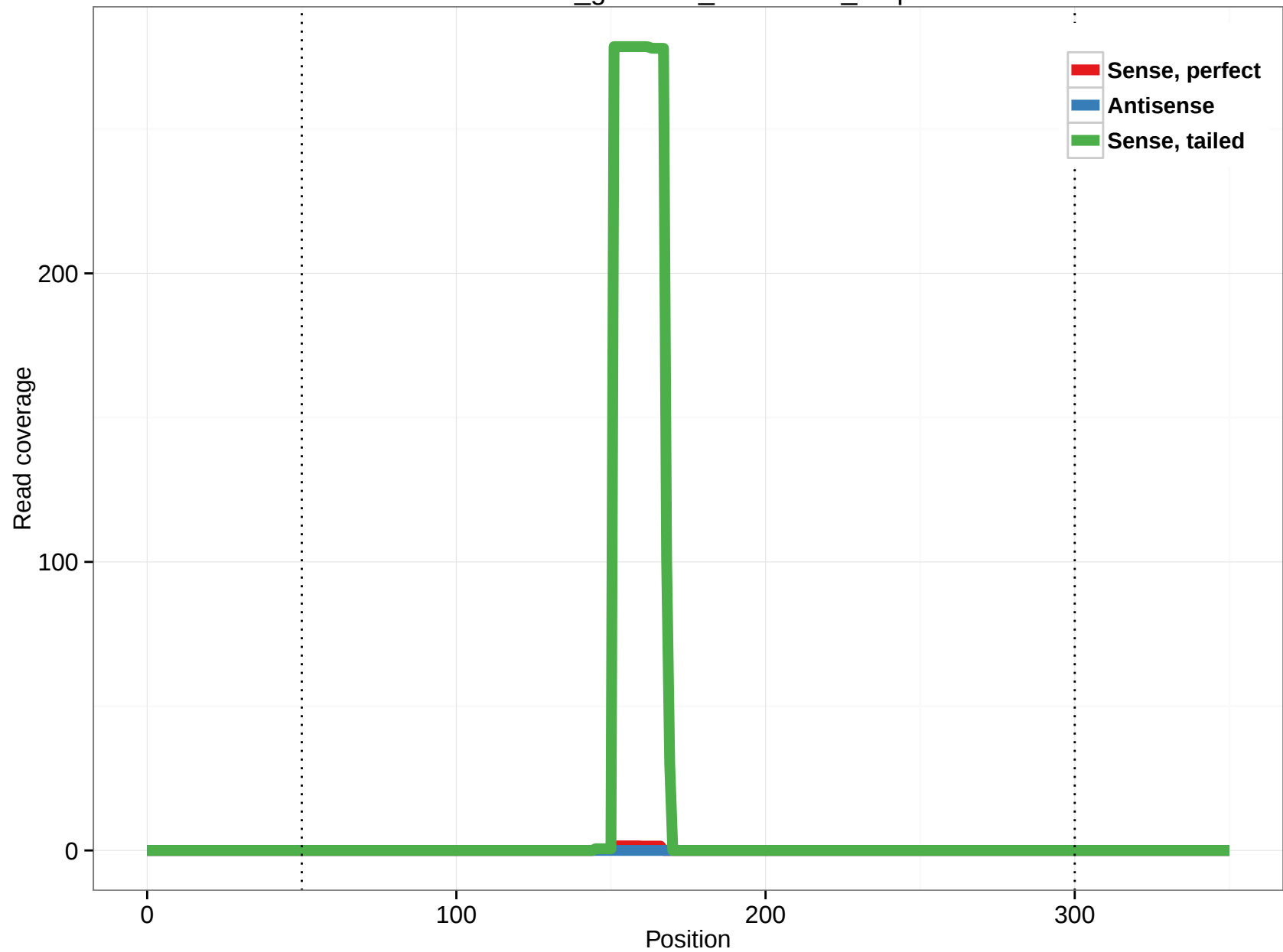
rheMac3_genscan_chr7.2614_0.3p
