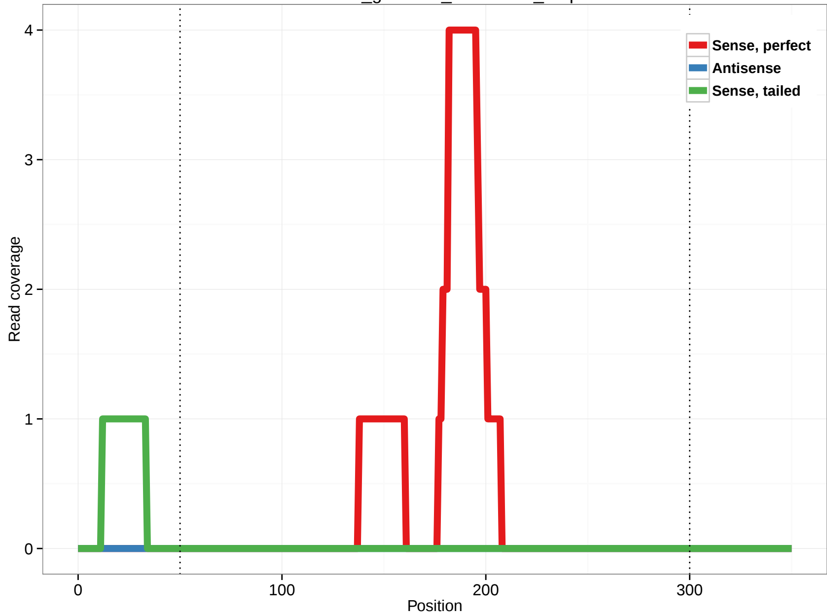
rheMac3_genscan_chr7.2606_9.3p
