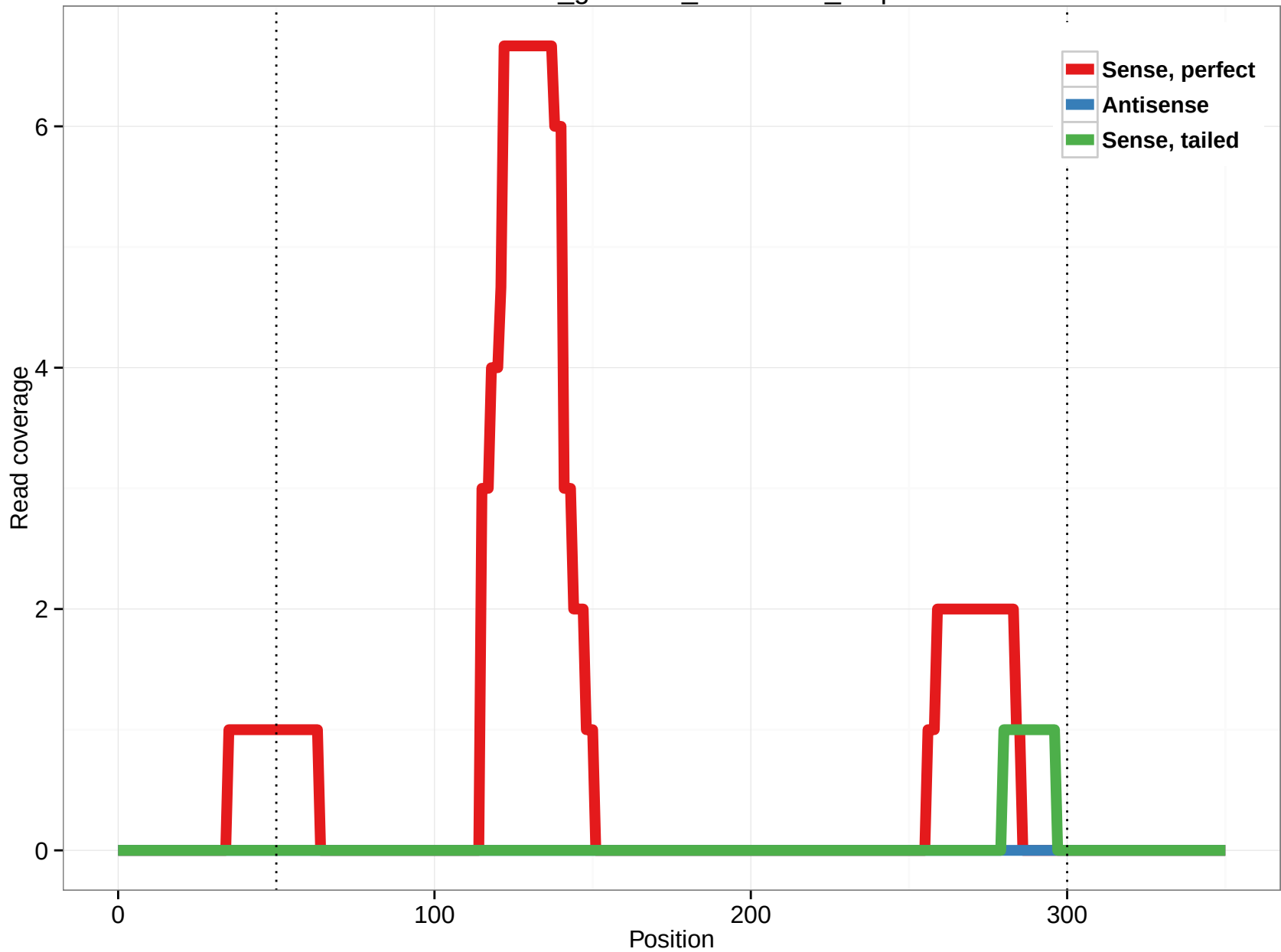
rheMac3_genscan_chr7.2602_2.5p
