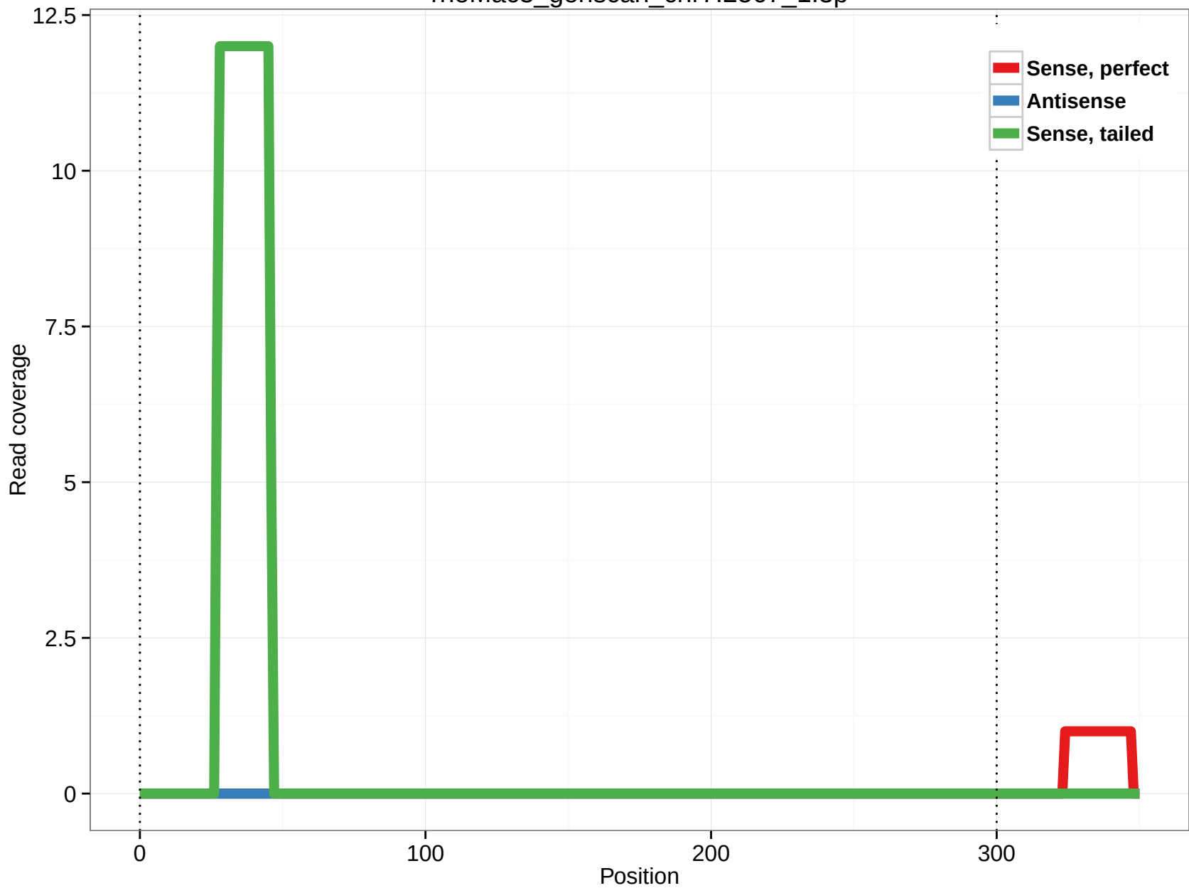
rheMac3_genscan_chr7.2567_1.3p
