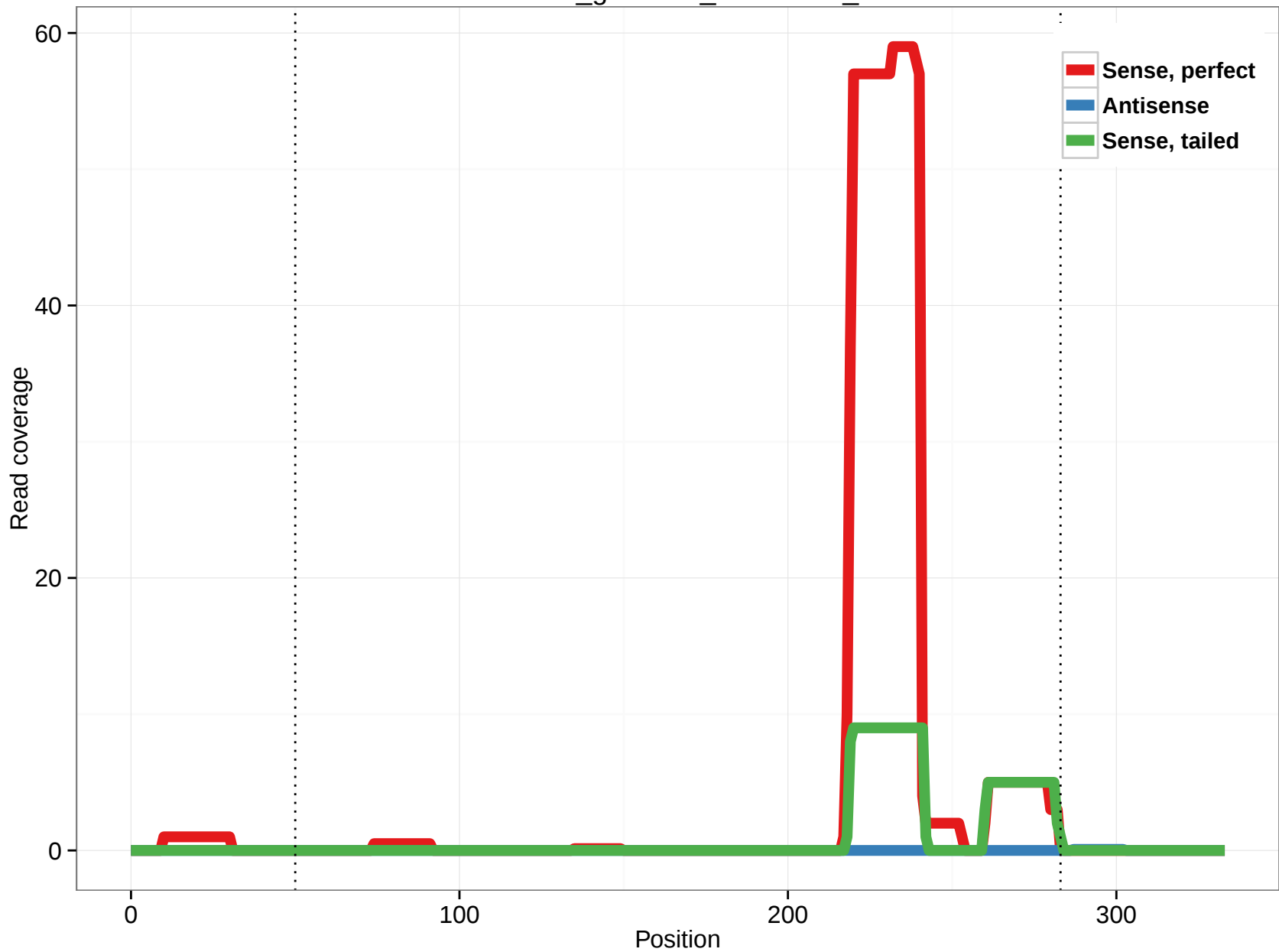
rheMac3_genscan_chr7.2533_18
