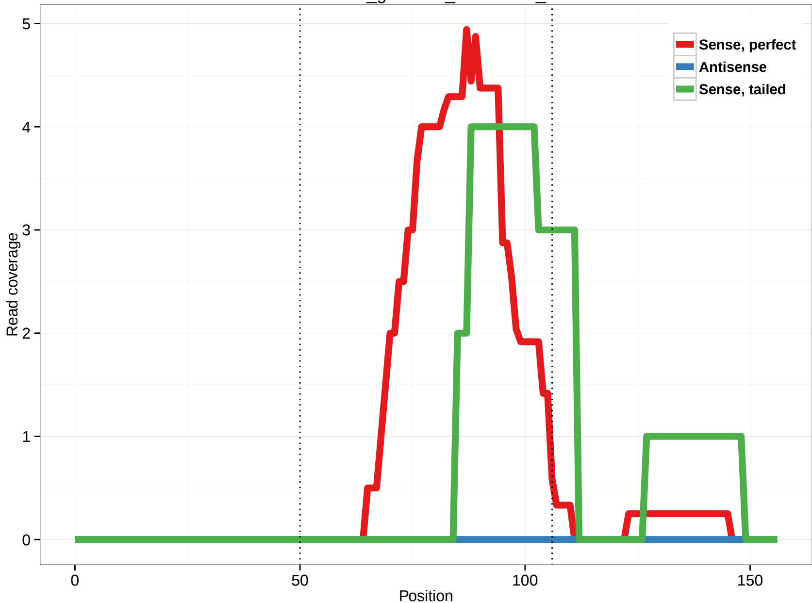
rheMac3_genscan_chr7.2457_4
