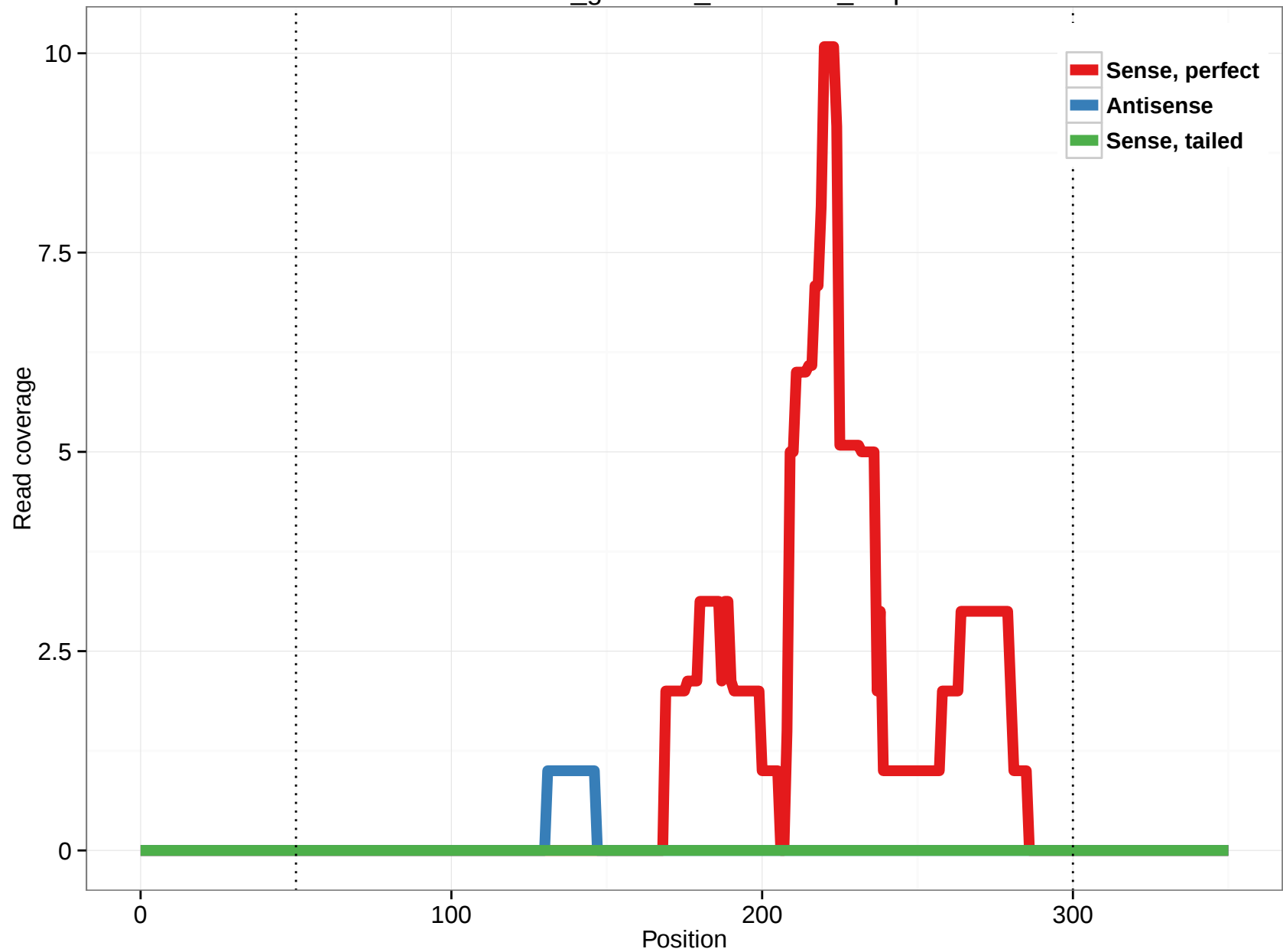
rheMac3_genscan_chr7.2105_1.5p
