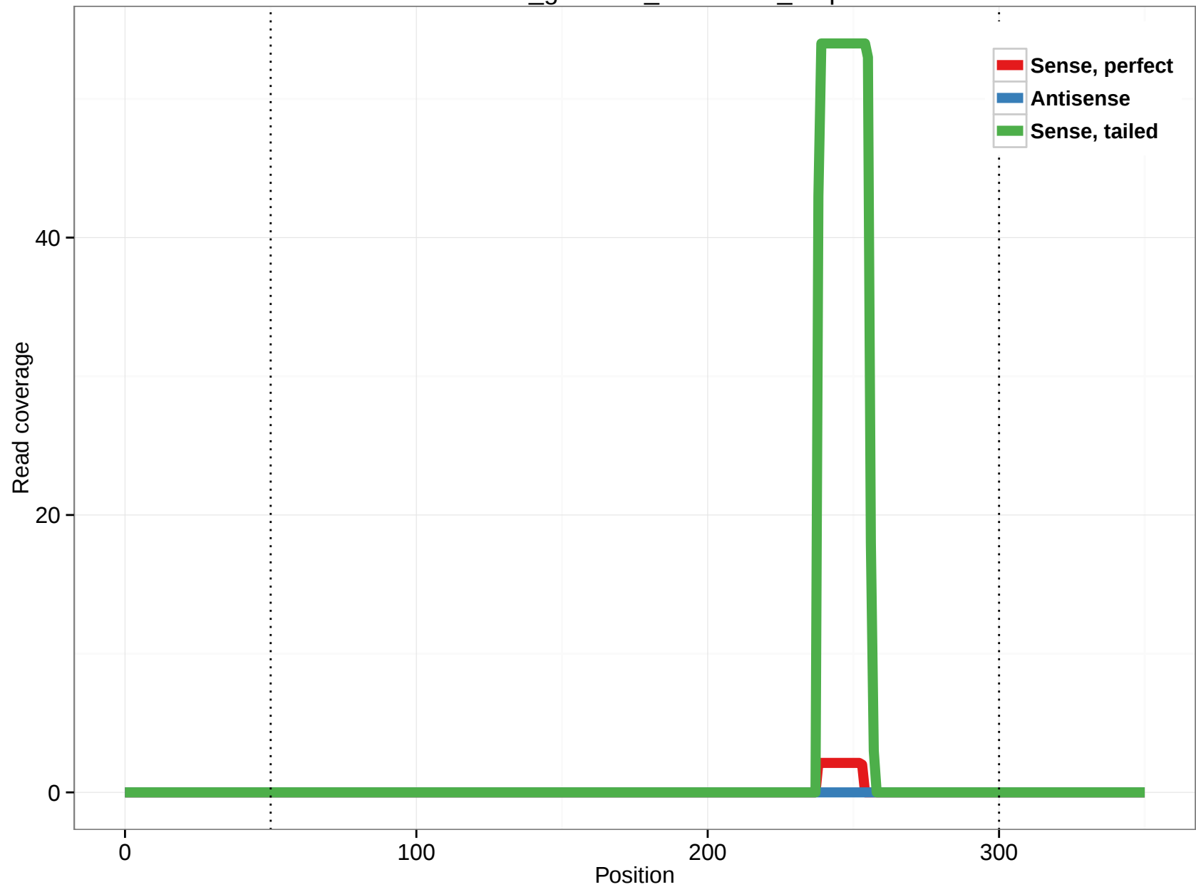
rheMac3_genscan_chr7.1996_4.5p
