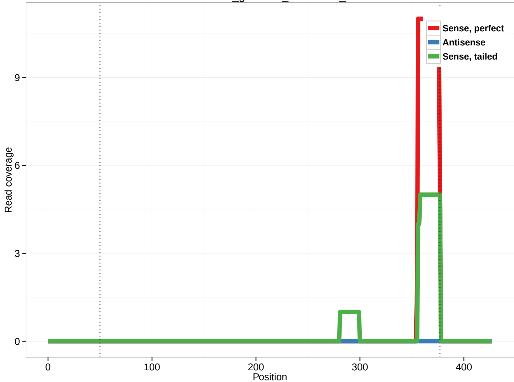
rheMac3_genscan_chr7.1991_3
