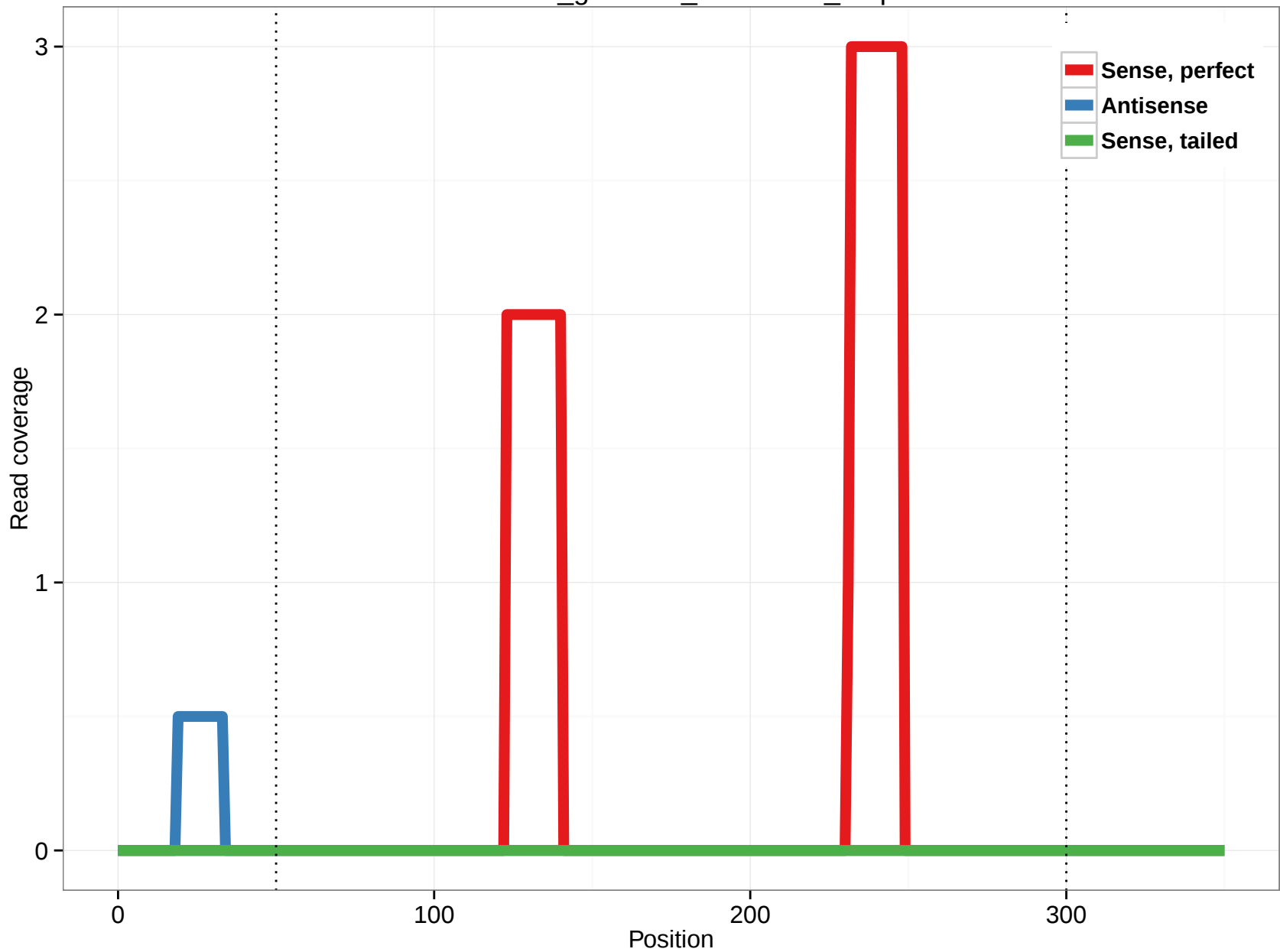
rheMac3_genscan_chr7.1935_1.3p
