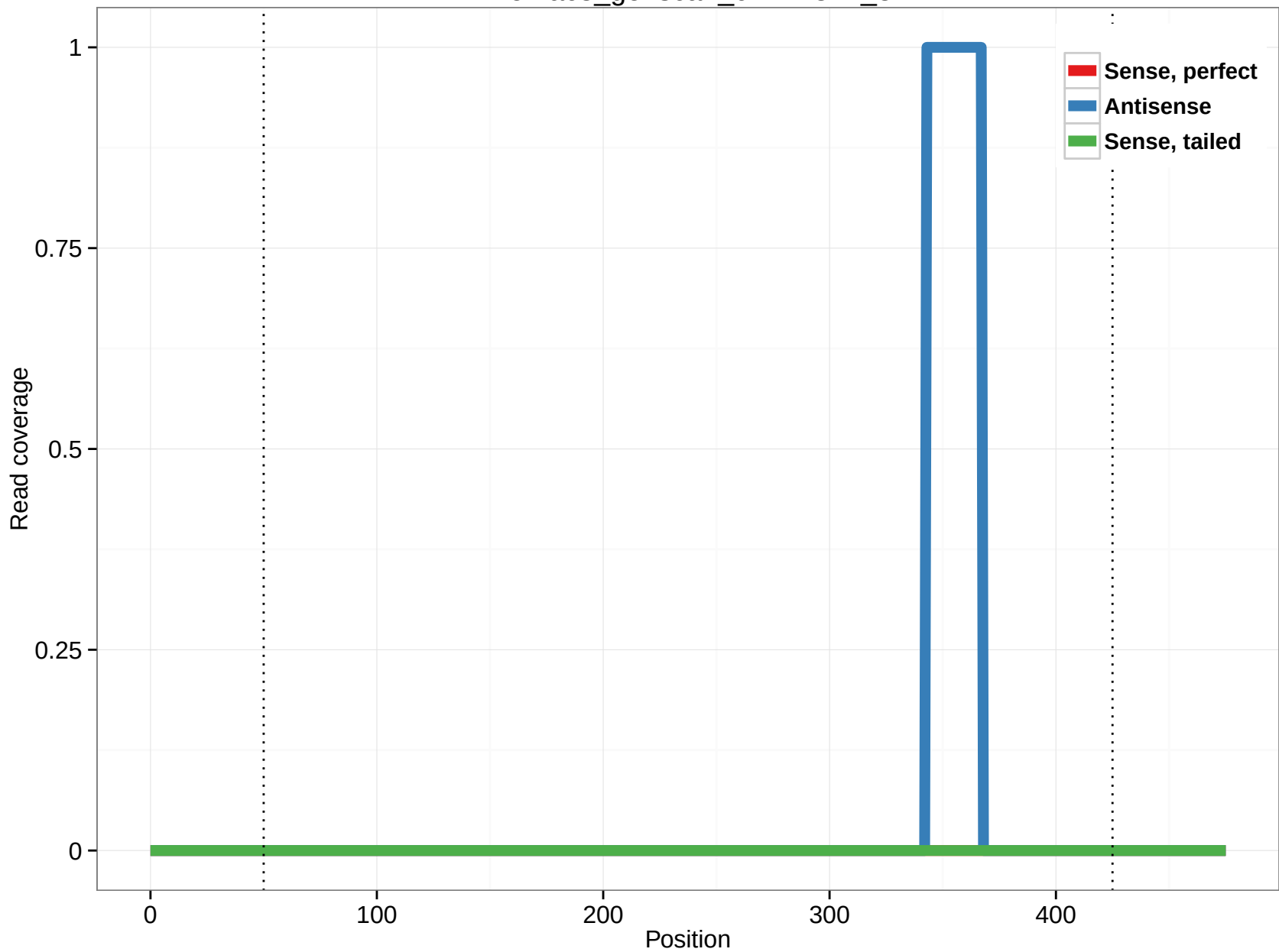
rheMac3_genscan_chr7.1841_3
