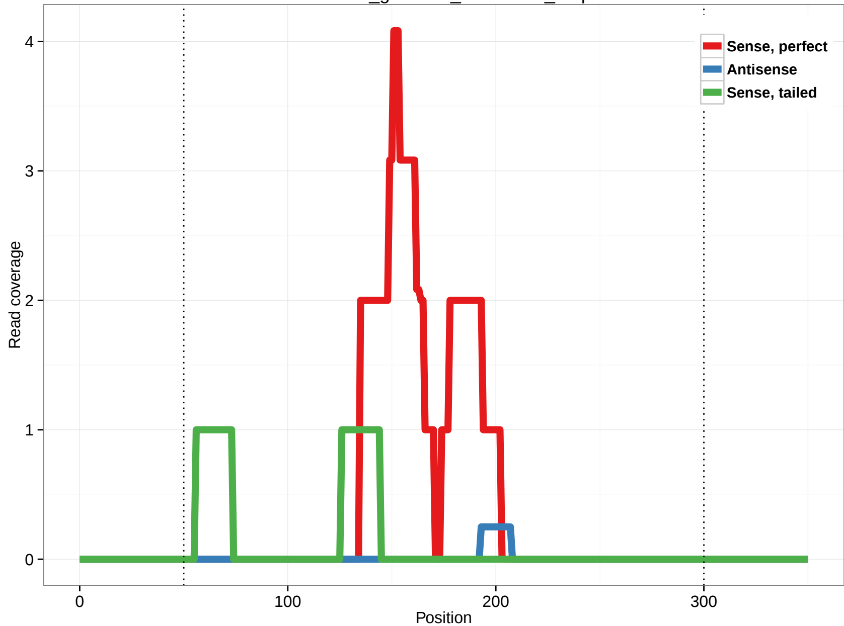
rheMac3_genscan_chr7.1784_1.3p
