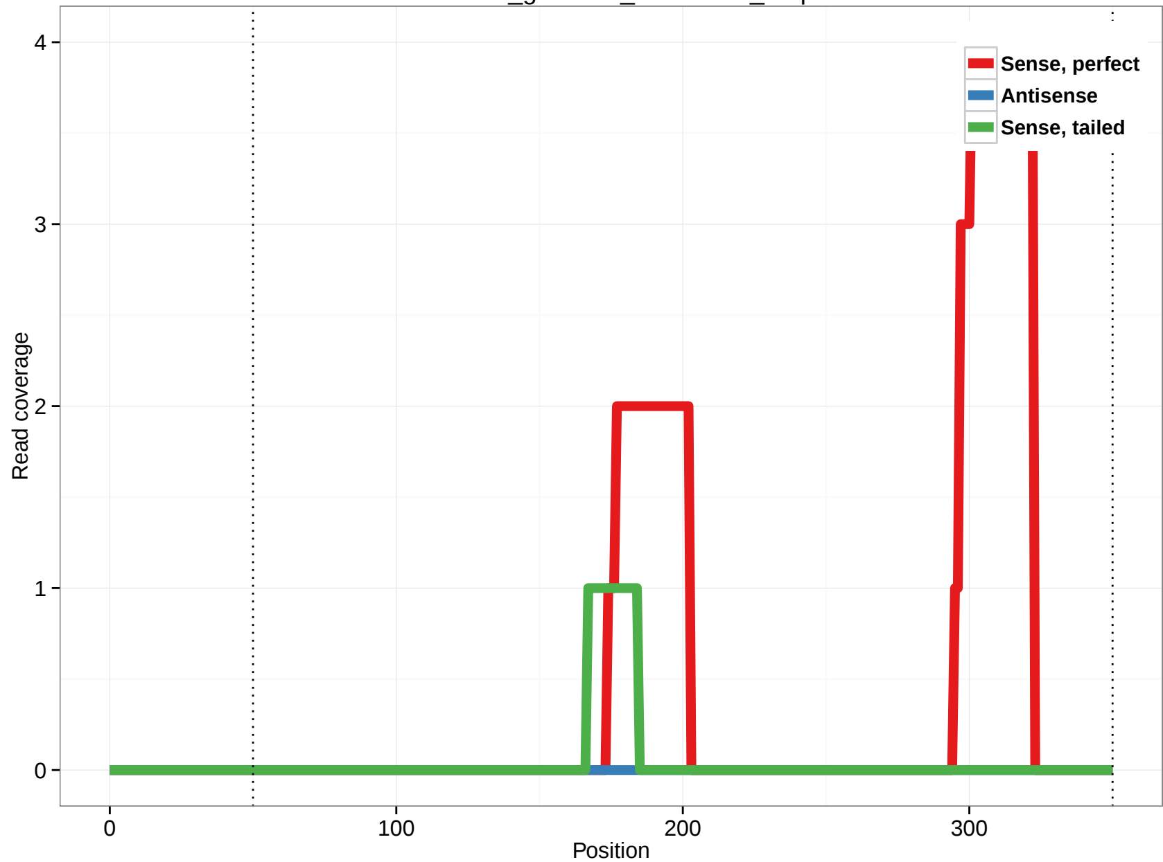
rheMac3_genscan_chr7.1776_8.5p
