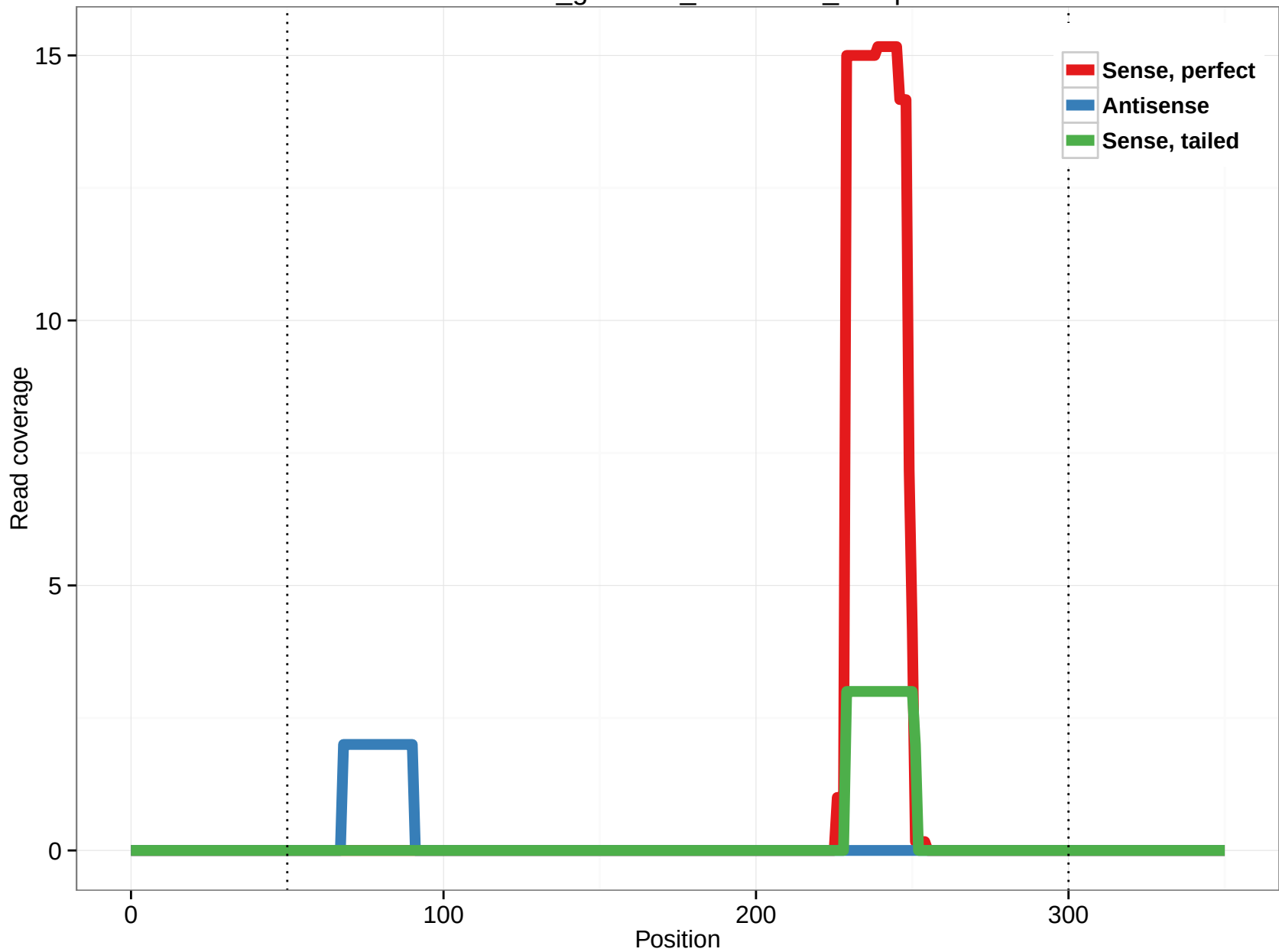
rheMac3_genscan_chr7.1776_11.3p
