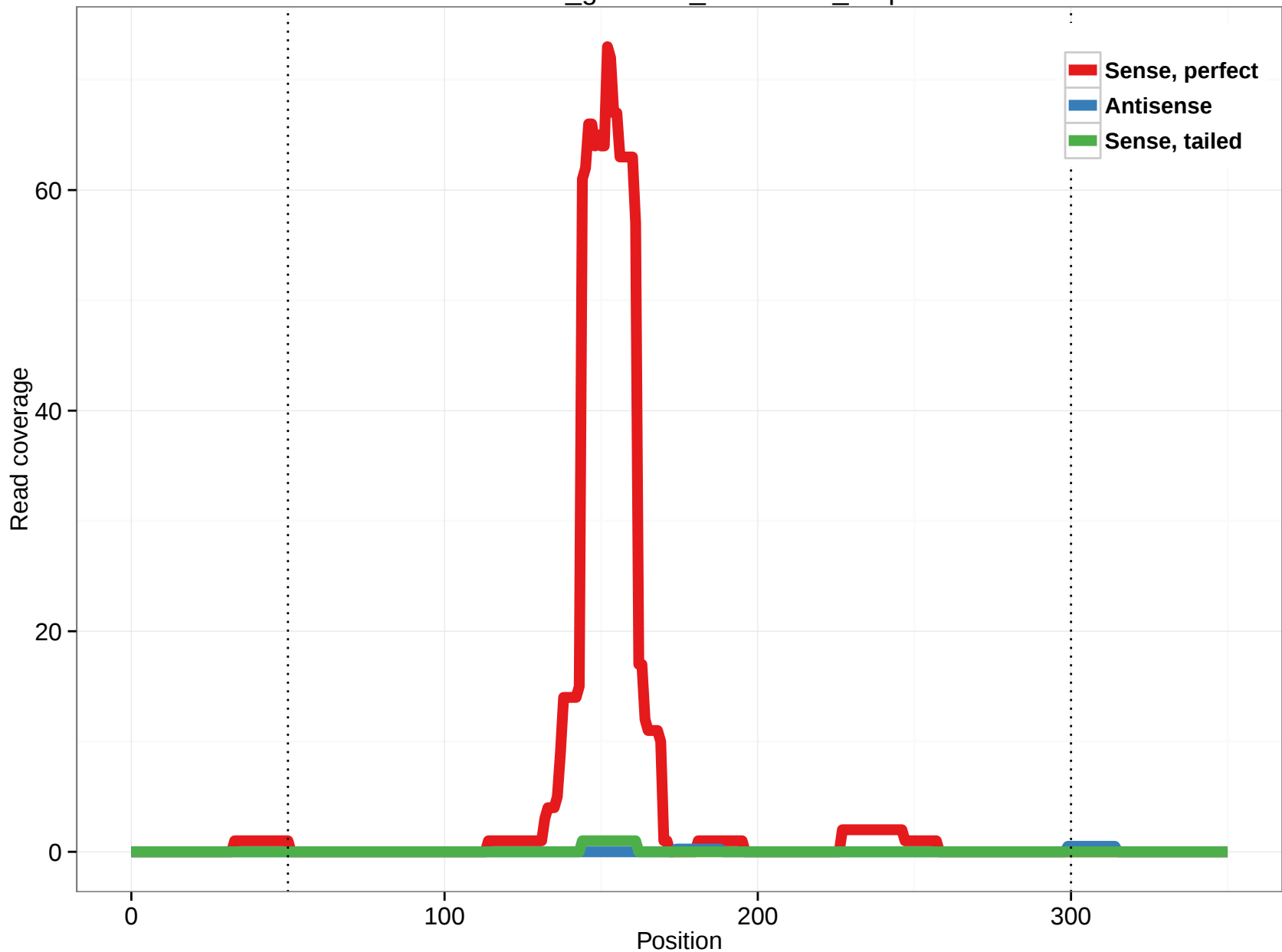
rheMac3_genscan_chr7.1757_5.5p
