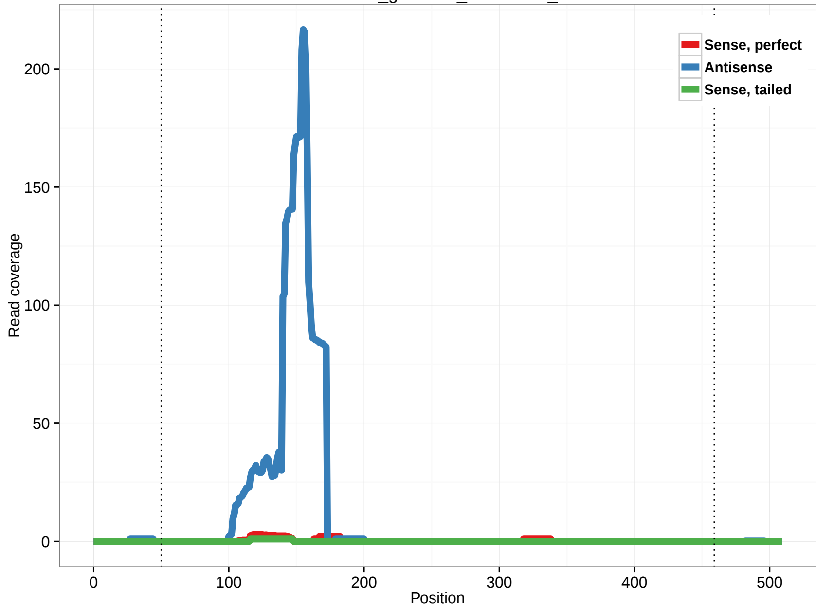
rheMac3_genscan_chr7.1755_5
