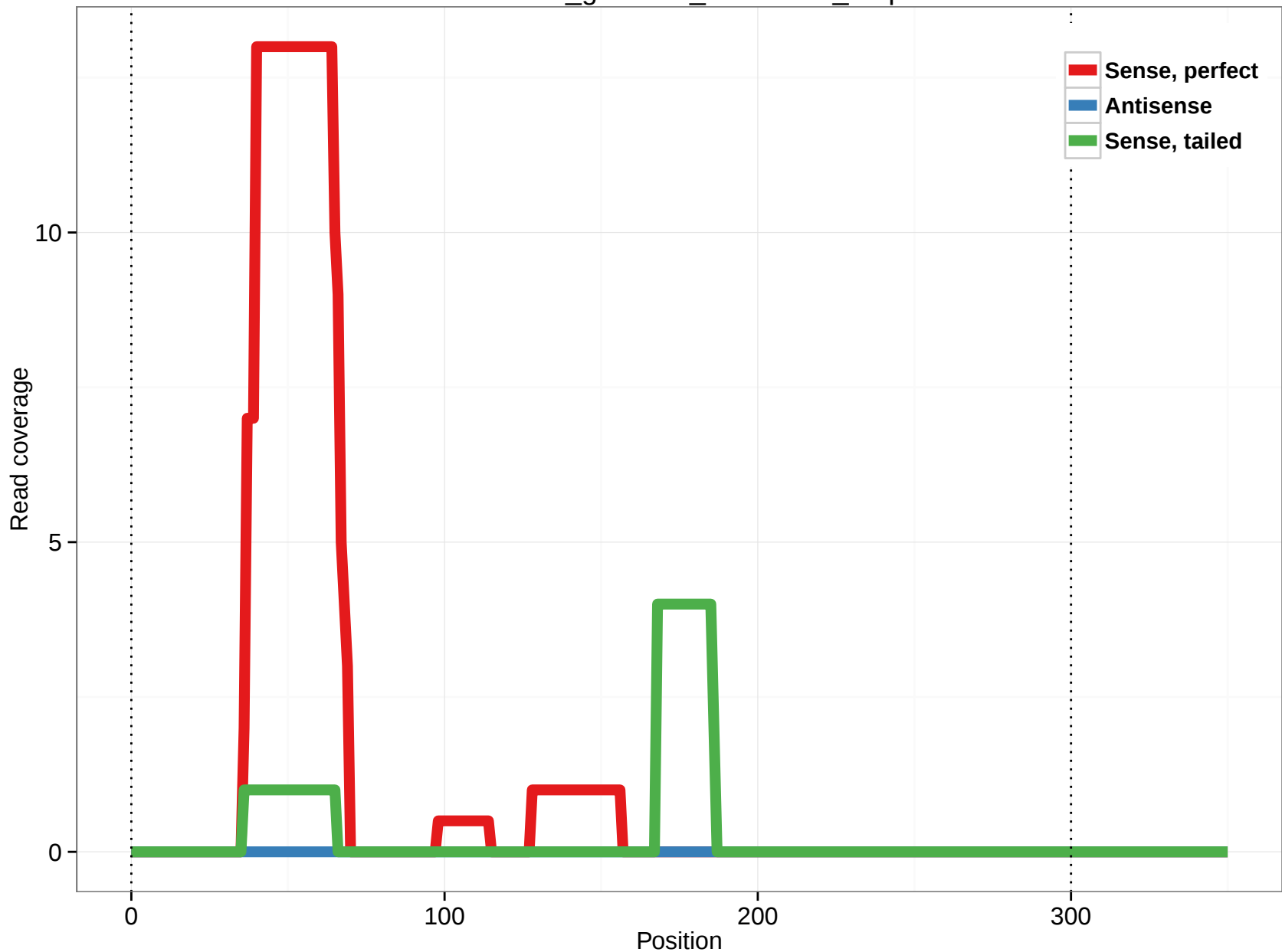
rheMac3_genscan_chr7.1749_5.3p
