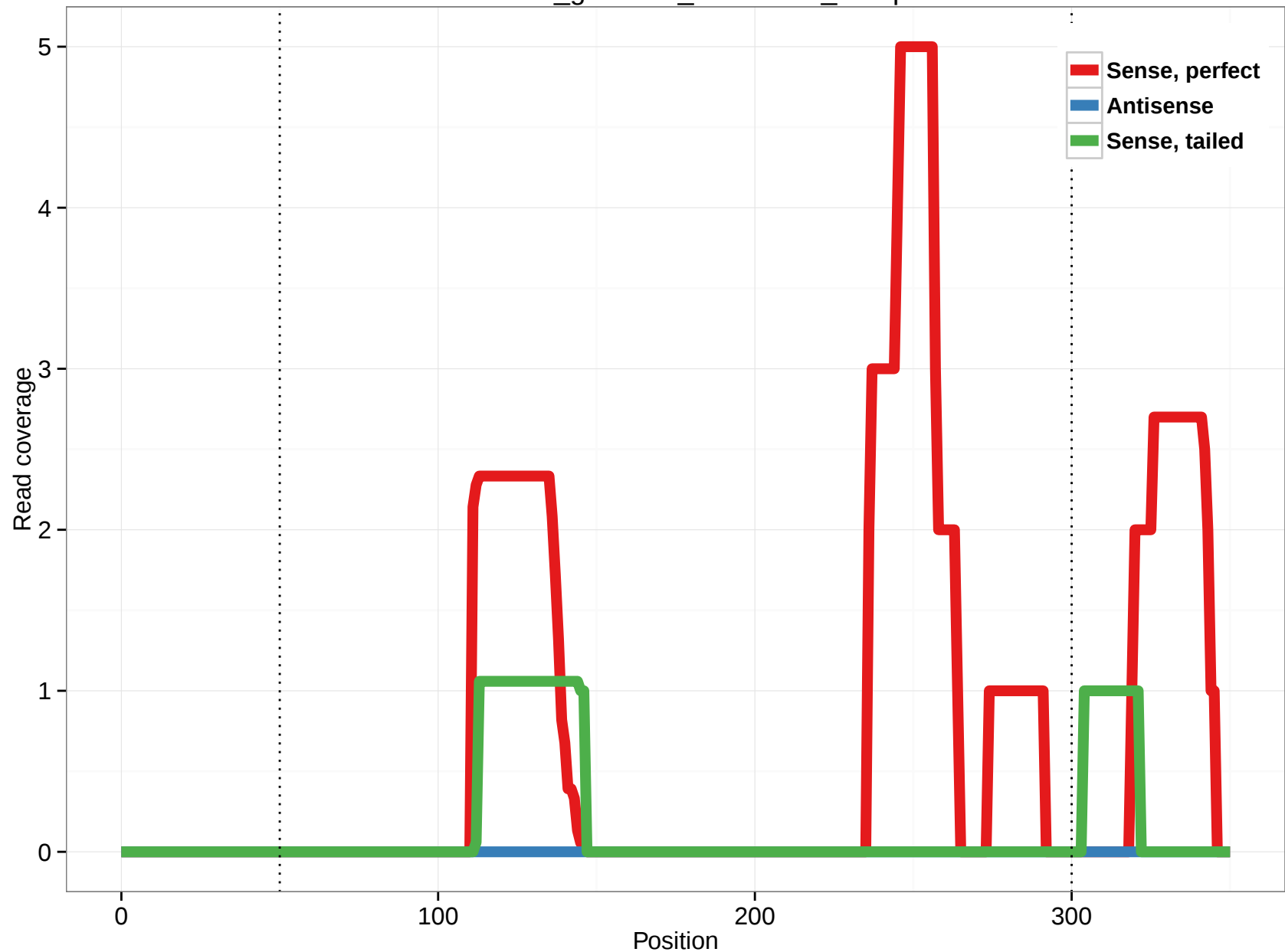
rheMac3_genscan_chr7.1711_34.3p
