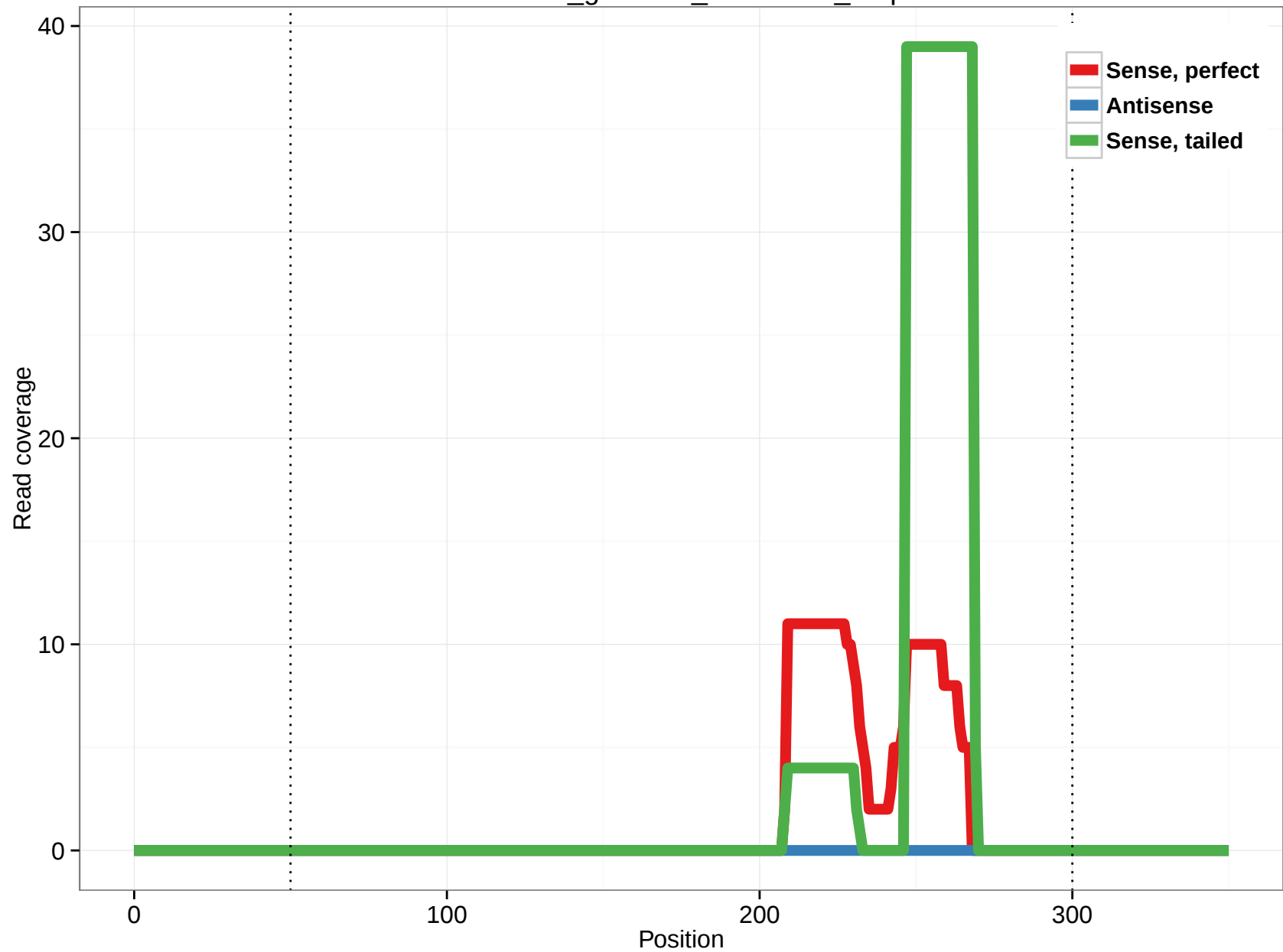
rheMac3_genscan_chr7.1698_4.3p
