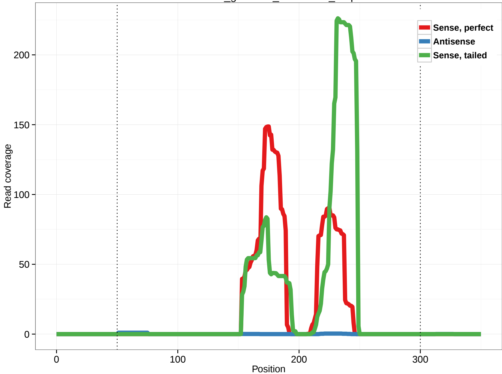
rheMac3_genscan_chr7.1686_7.5p
