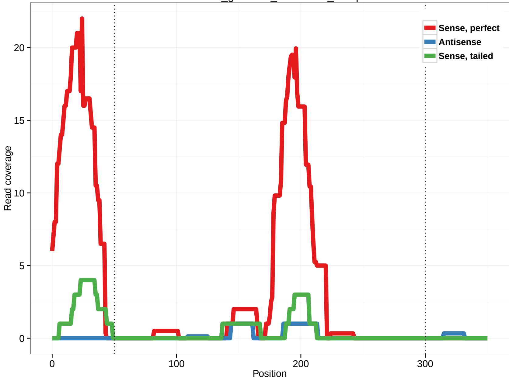
rheMac3_genscan_chr7.1580_11.5p
