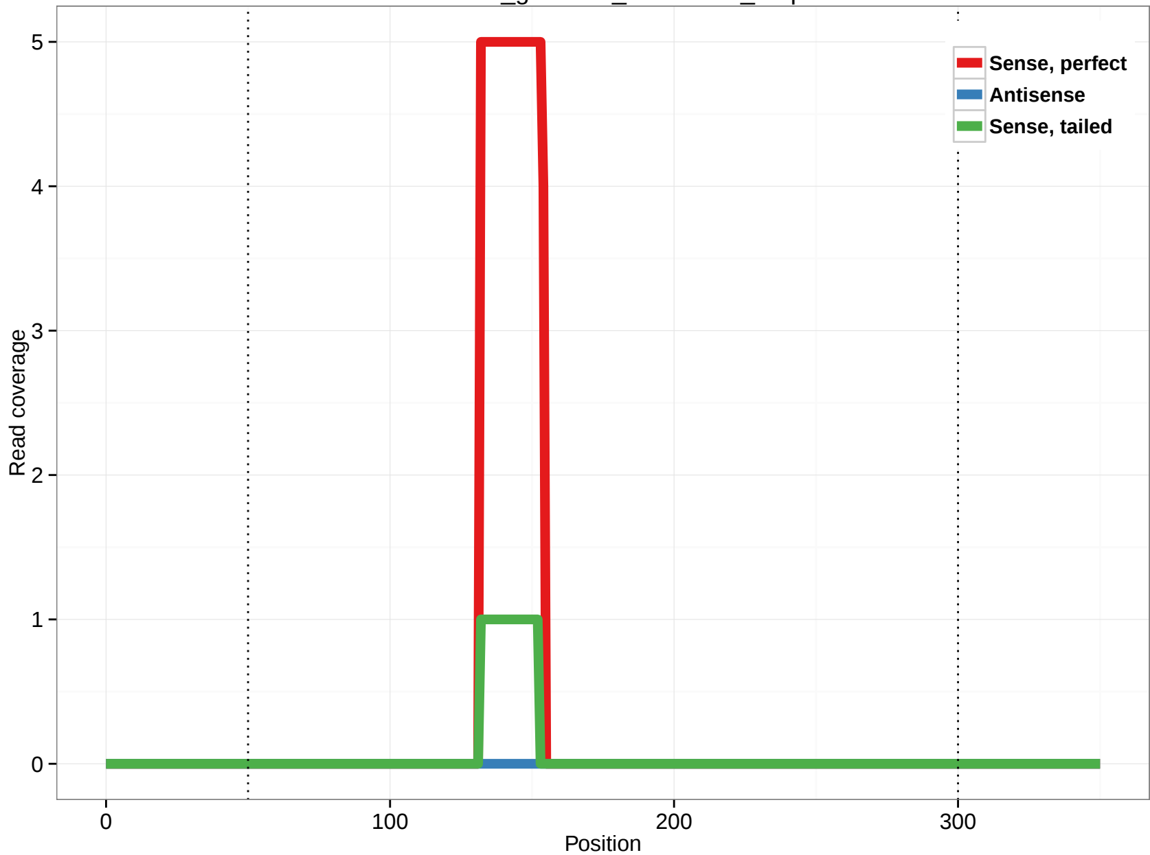
rheMac3_genscan_chr7.1570_4.5p
