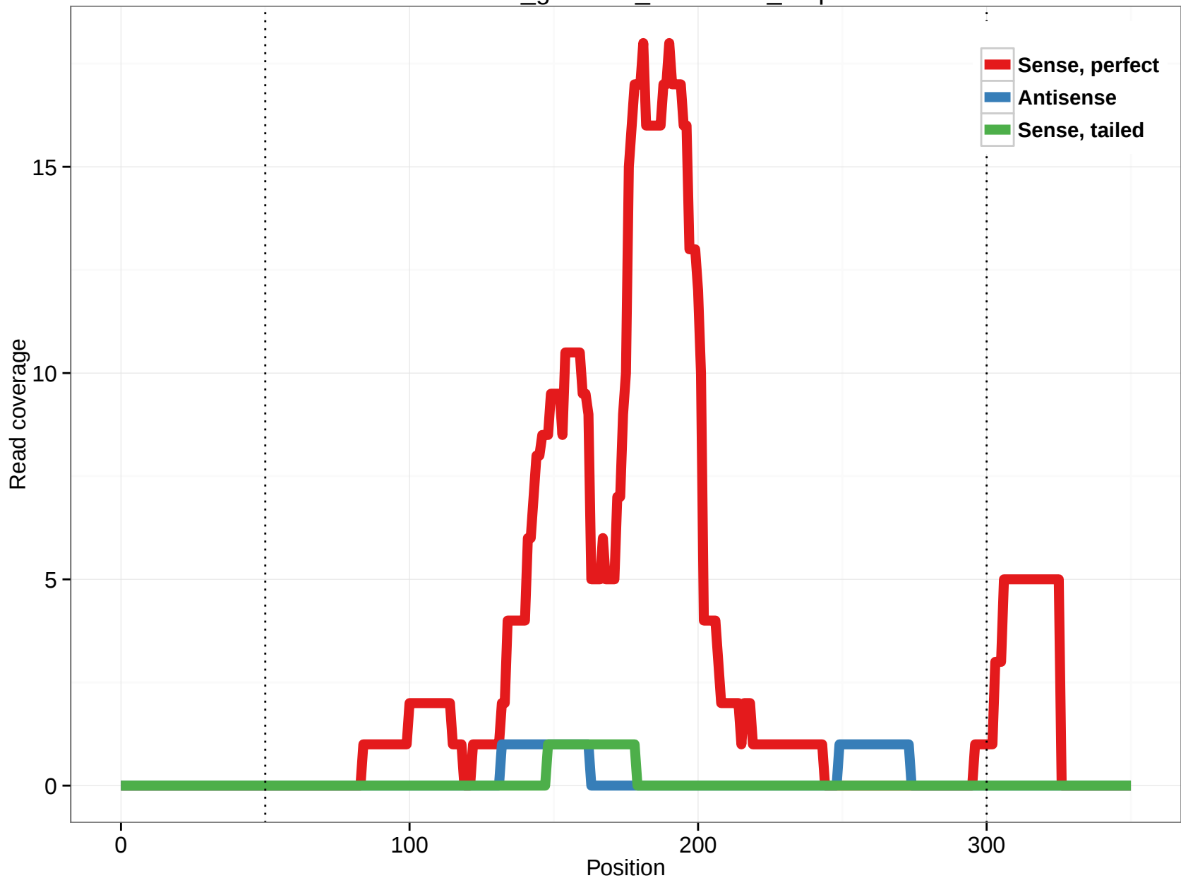
rheMac3_genscan_chr7.1561_1.5p
