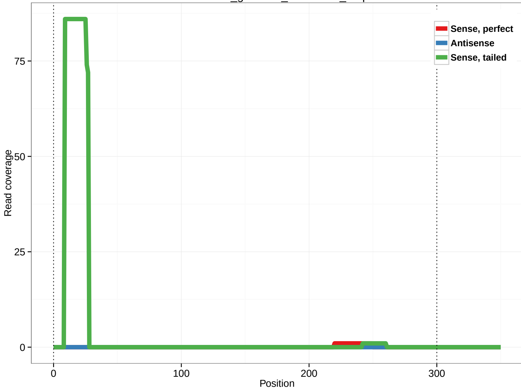
rheMac3_genscan_chr7.1554_3.3p
