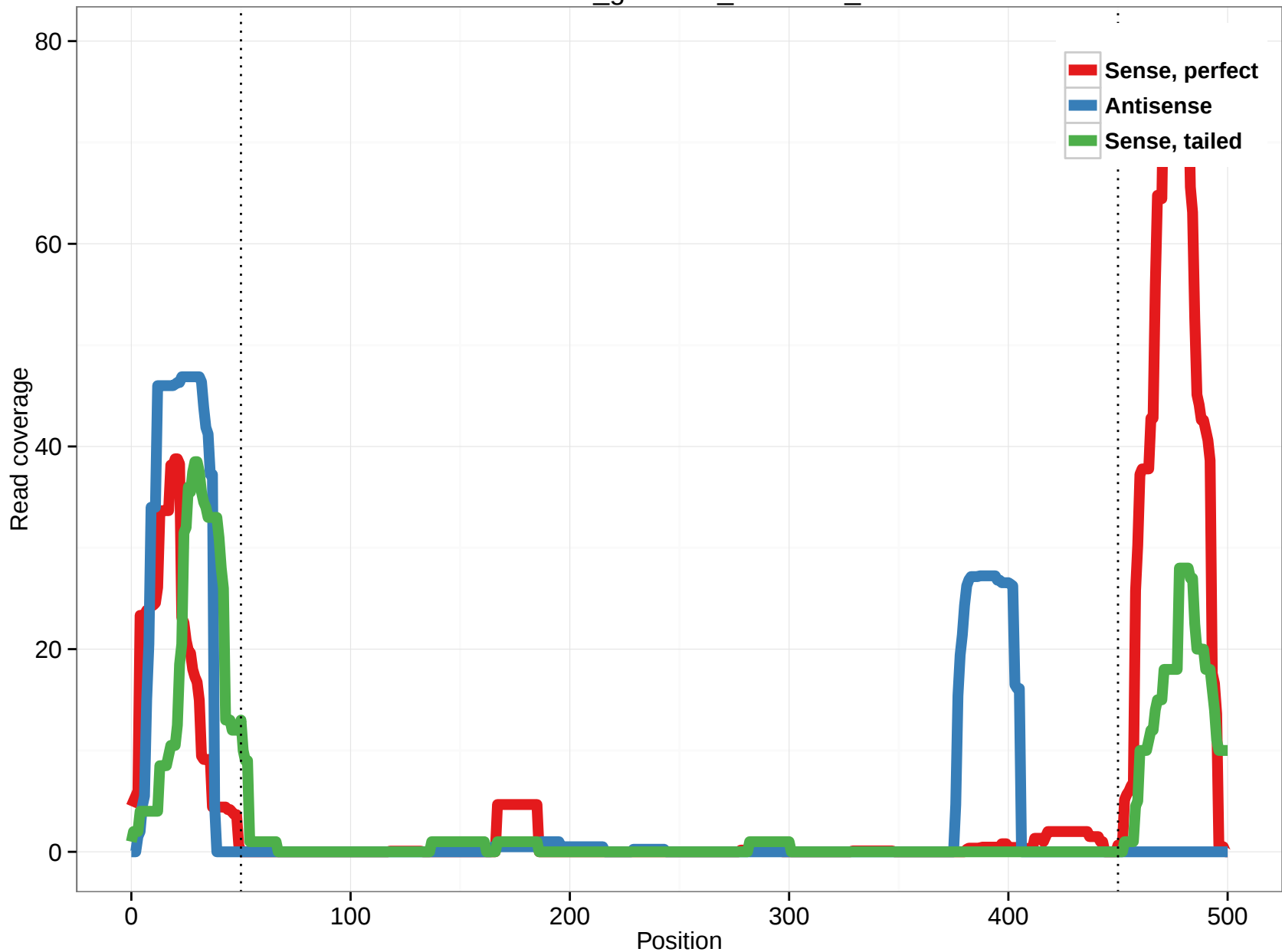
rheMac3_genscan_chr7.151_6
