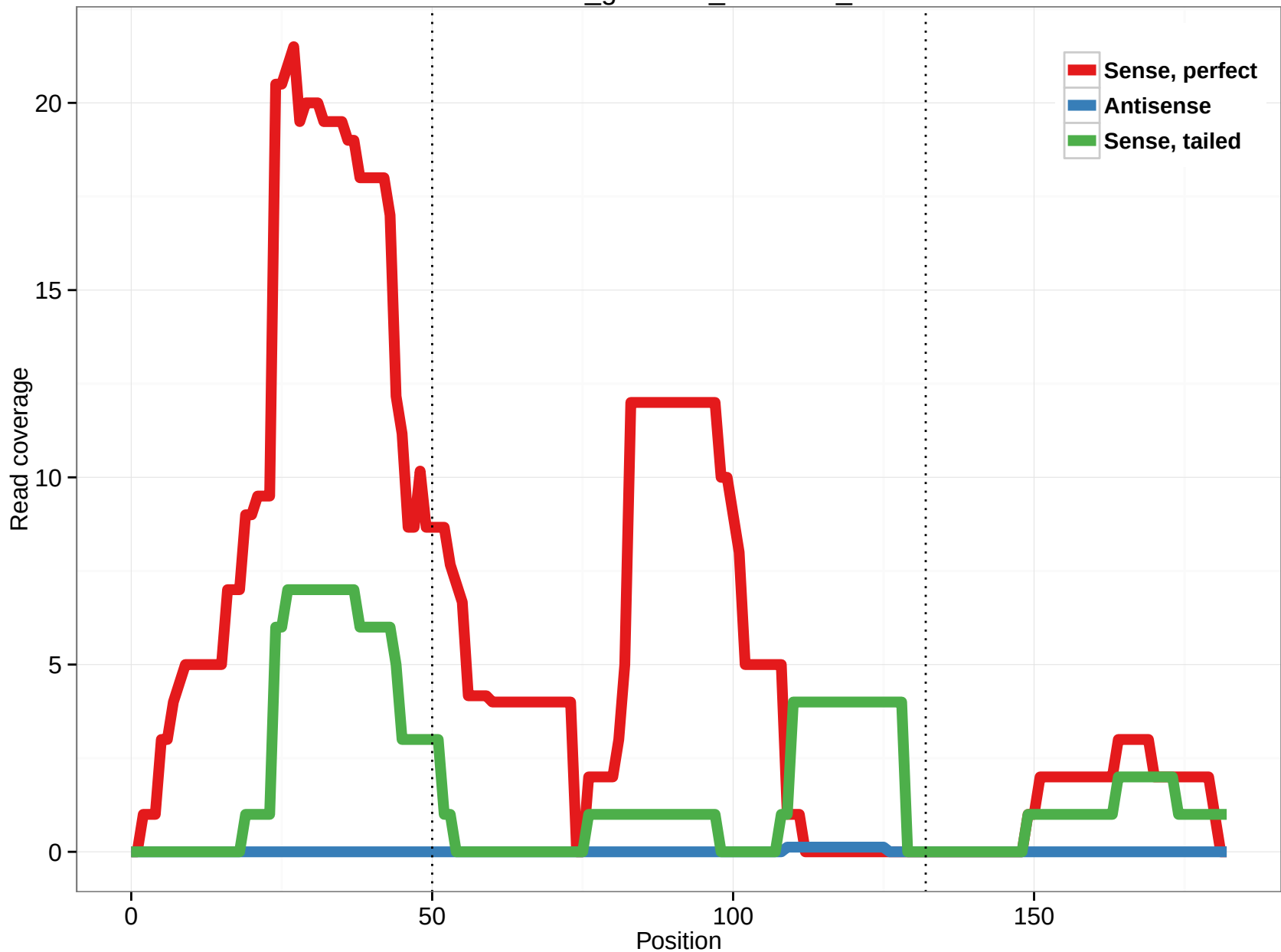
rheMac3_genscan_chr7.151_12
