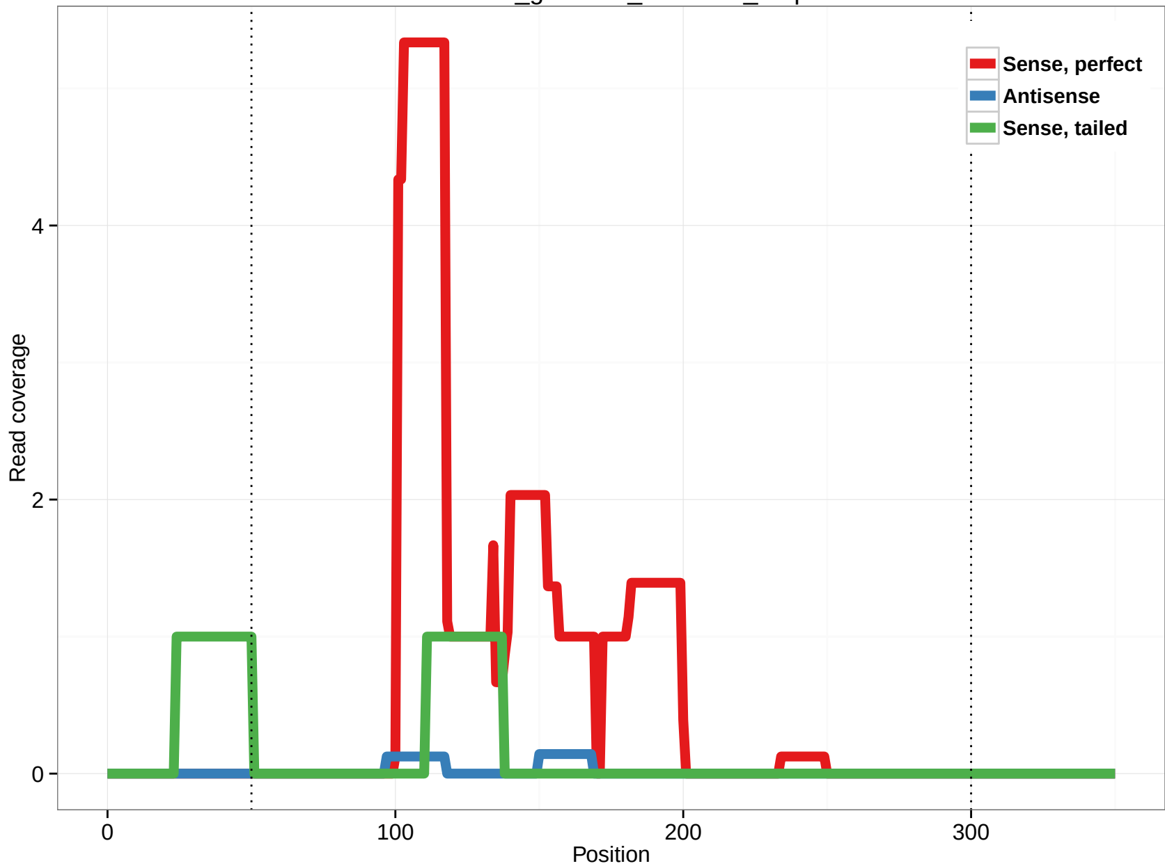
rheMac3_genscan_chr7.151_1.5p
