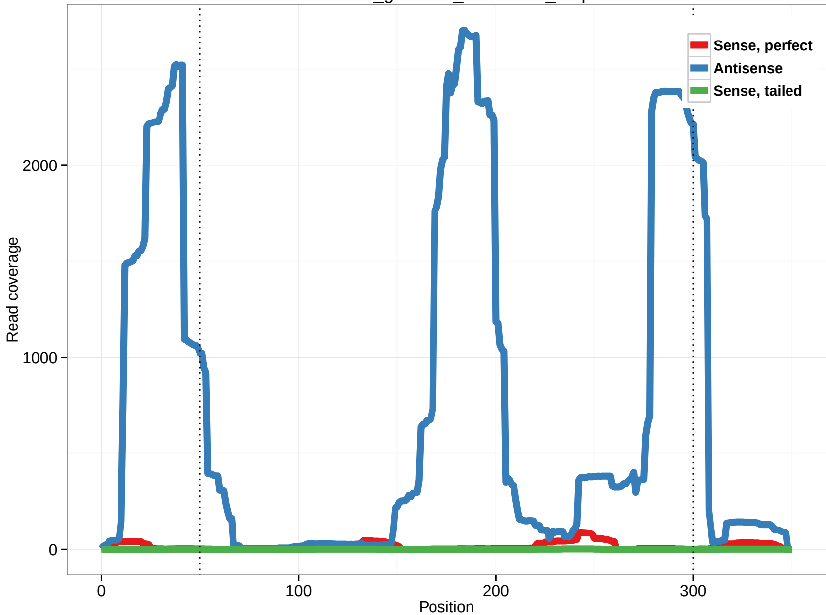
rheMac3_genscan_chr7.1515_5.5p
