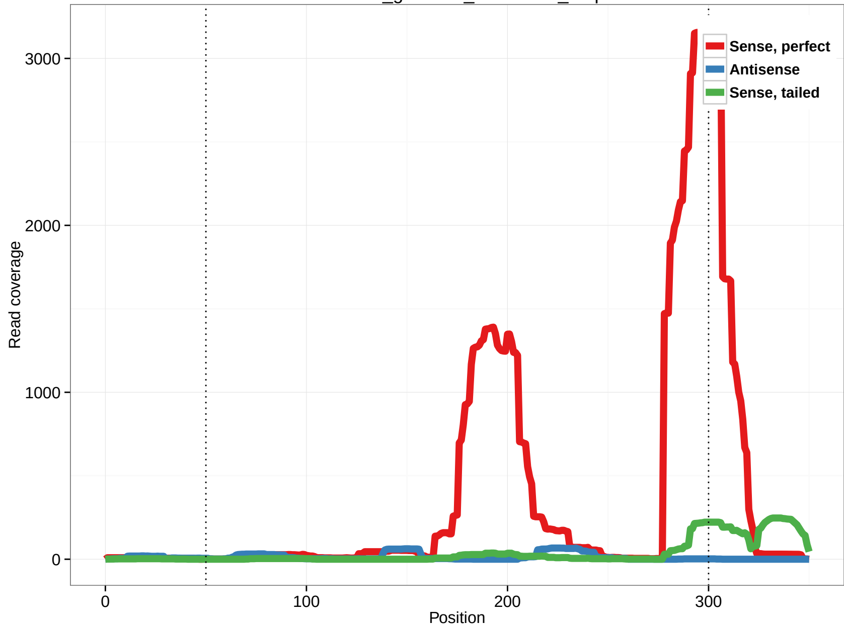
rheMac3_genscan_chr7.1442_0.5p
