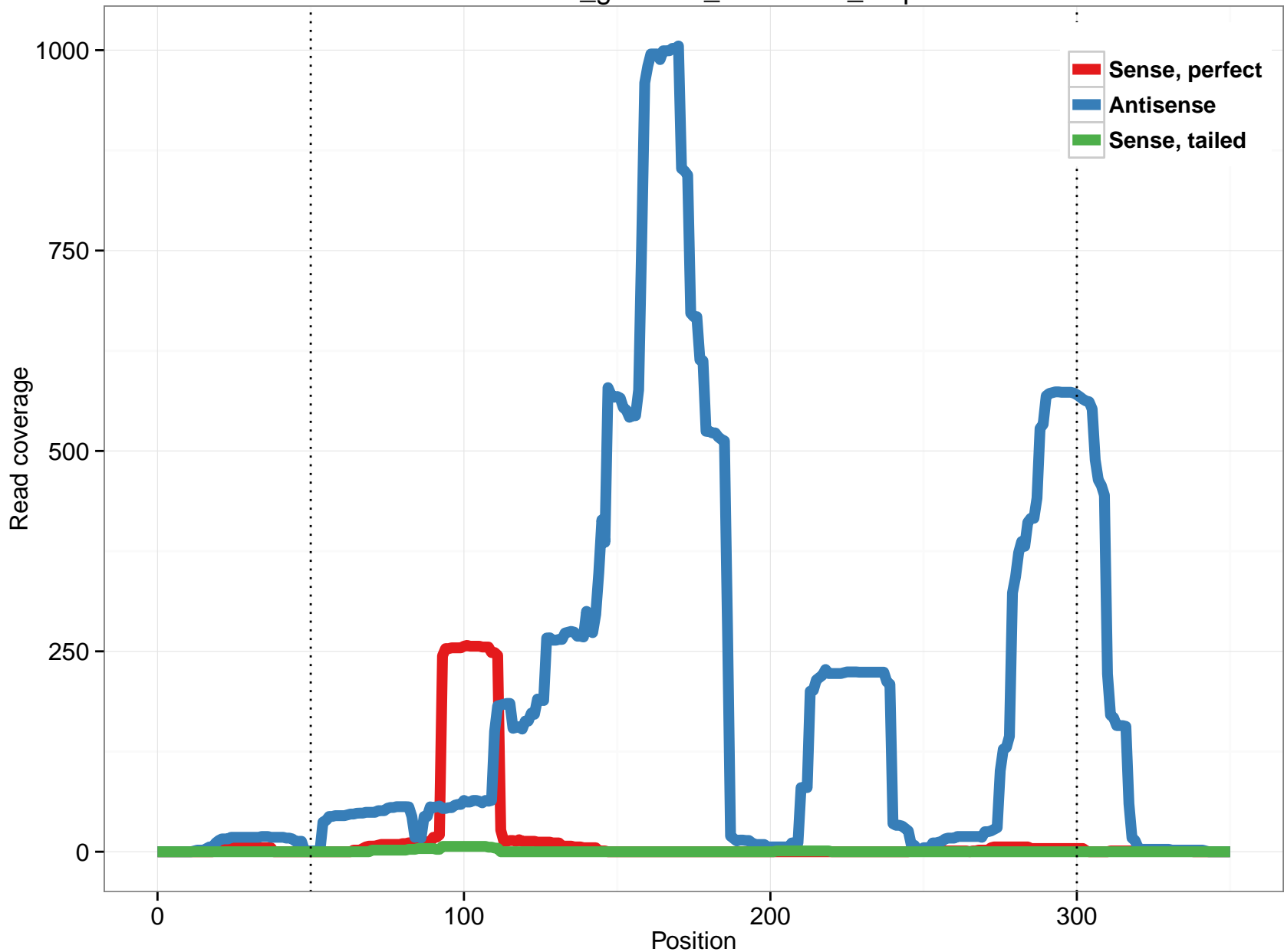
rheMac3_genscan_chr7.1421_7.5p
