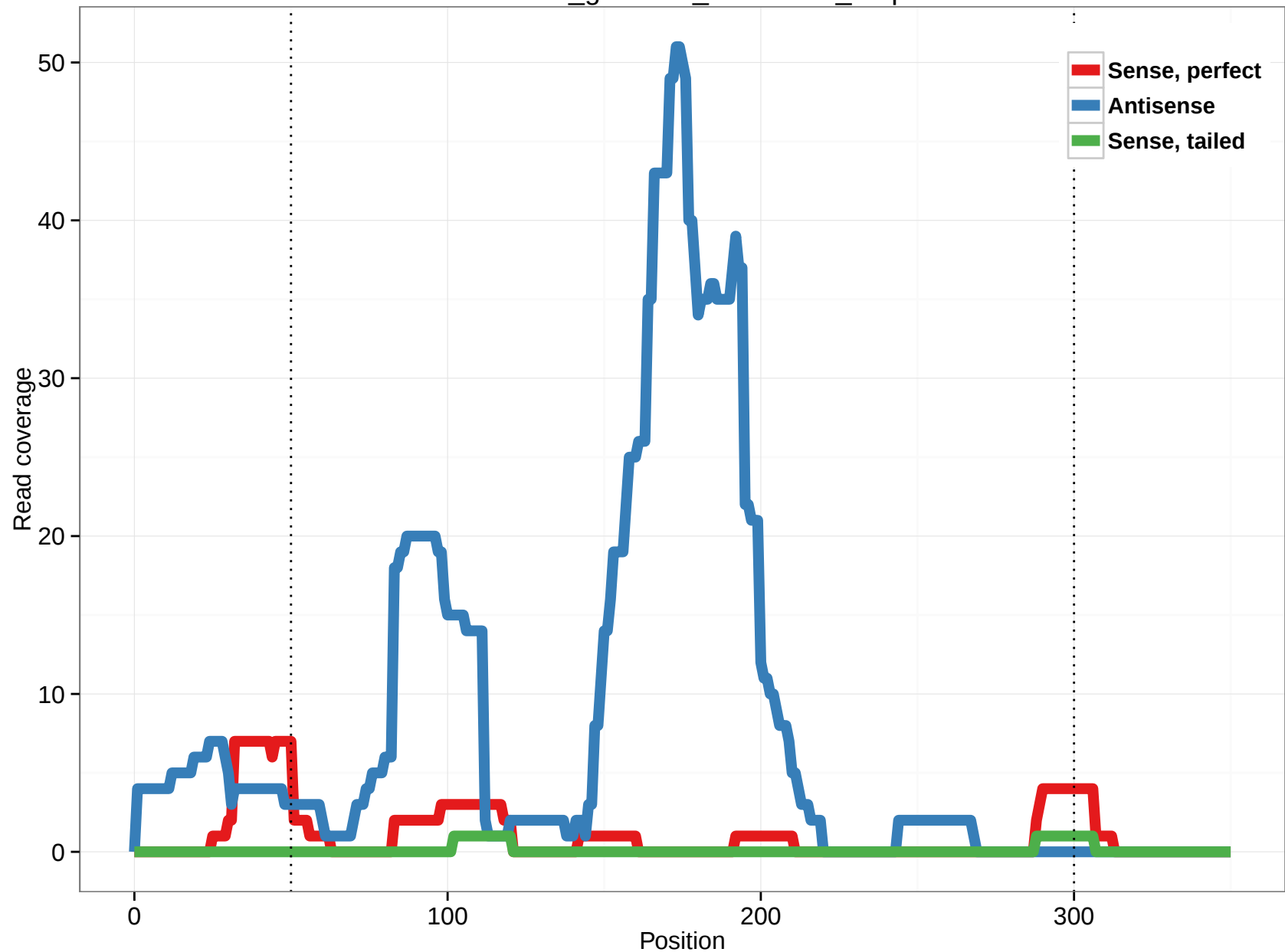
rheMac3_genscan_chr7.1421_4.5p
