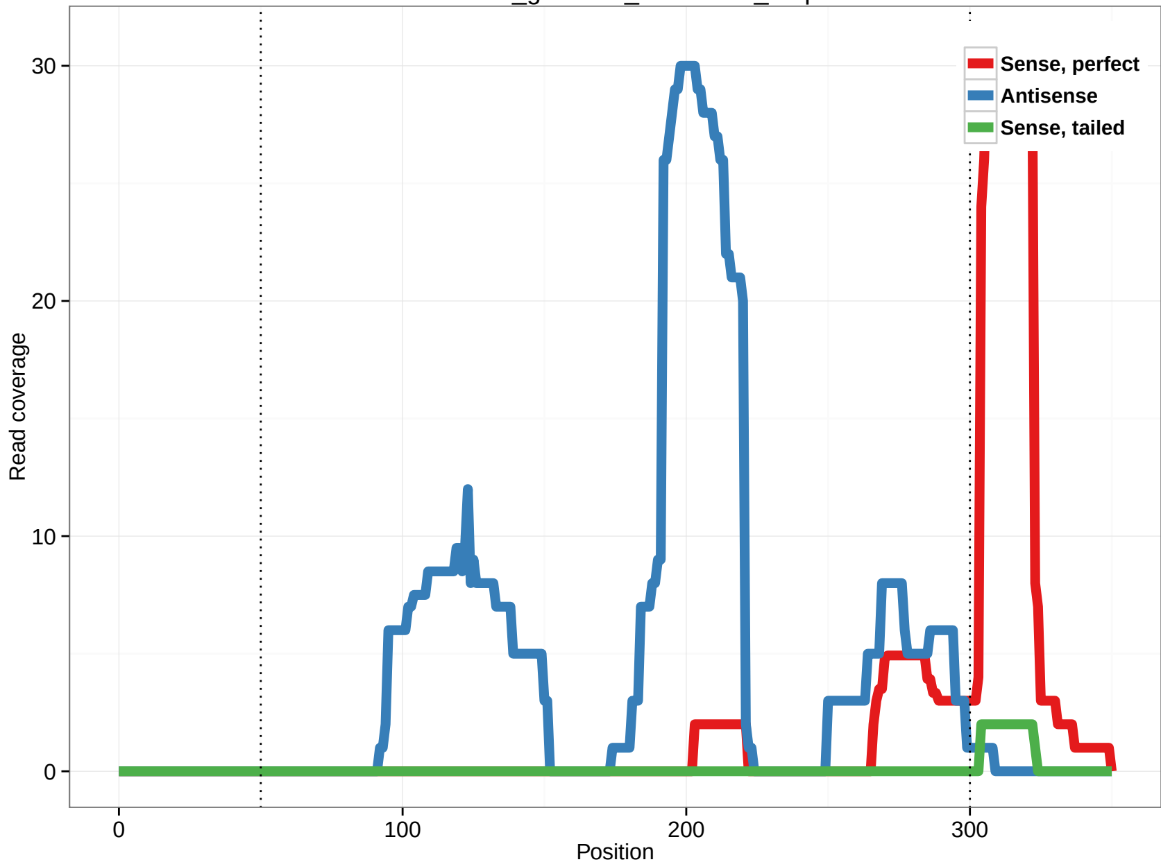
rheMac3_genscan_chr7.1421_4.3p
