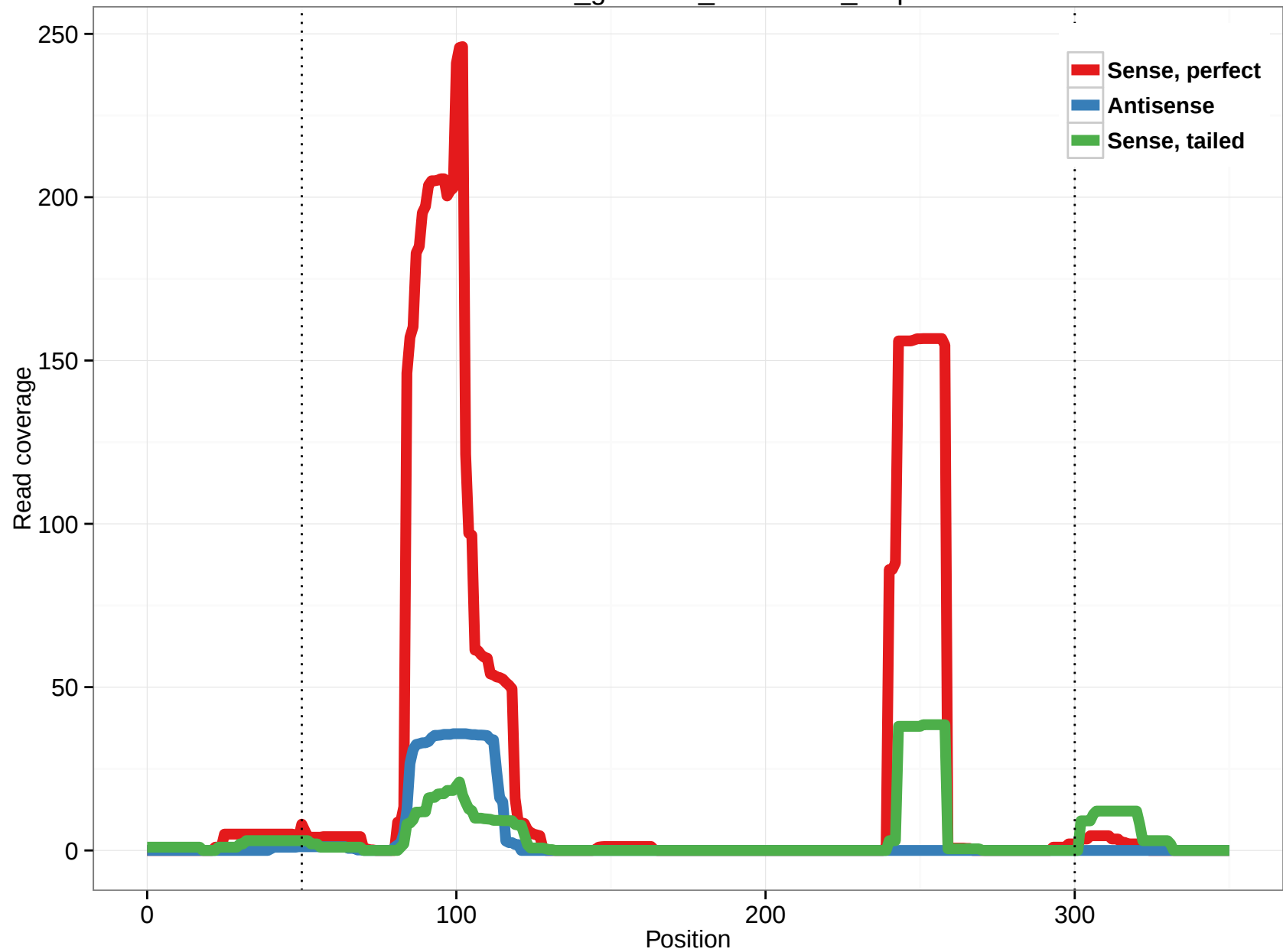
rheMac3_genscan_chr7.1409_2.5p
