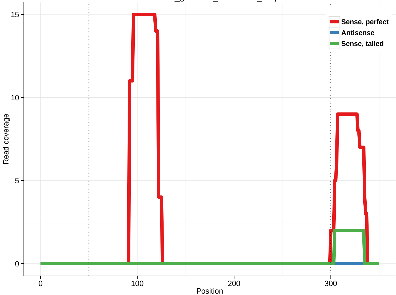
rheMac3_genscan_chr7.1375_6.3p
