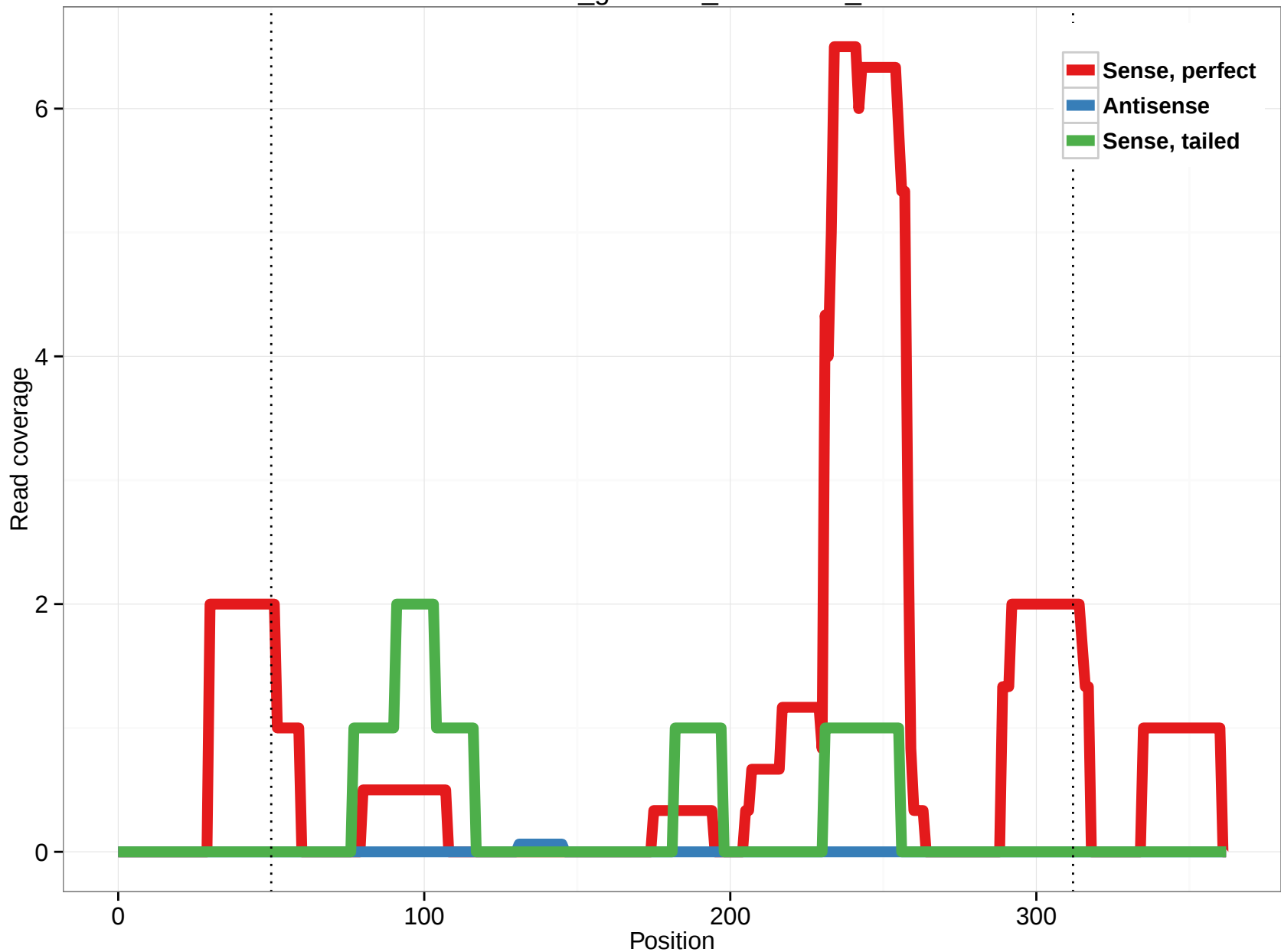
rheMac3_genscan_chr7.1291_3
