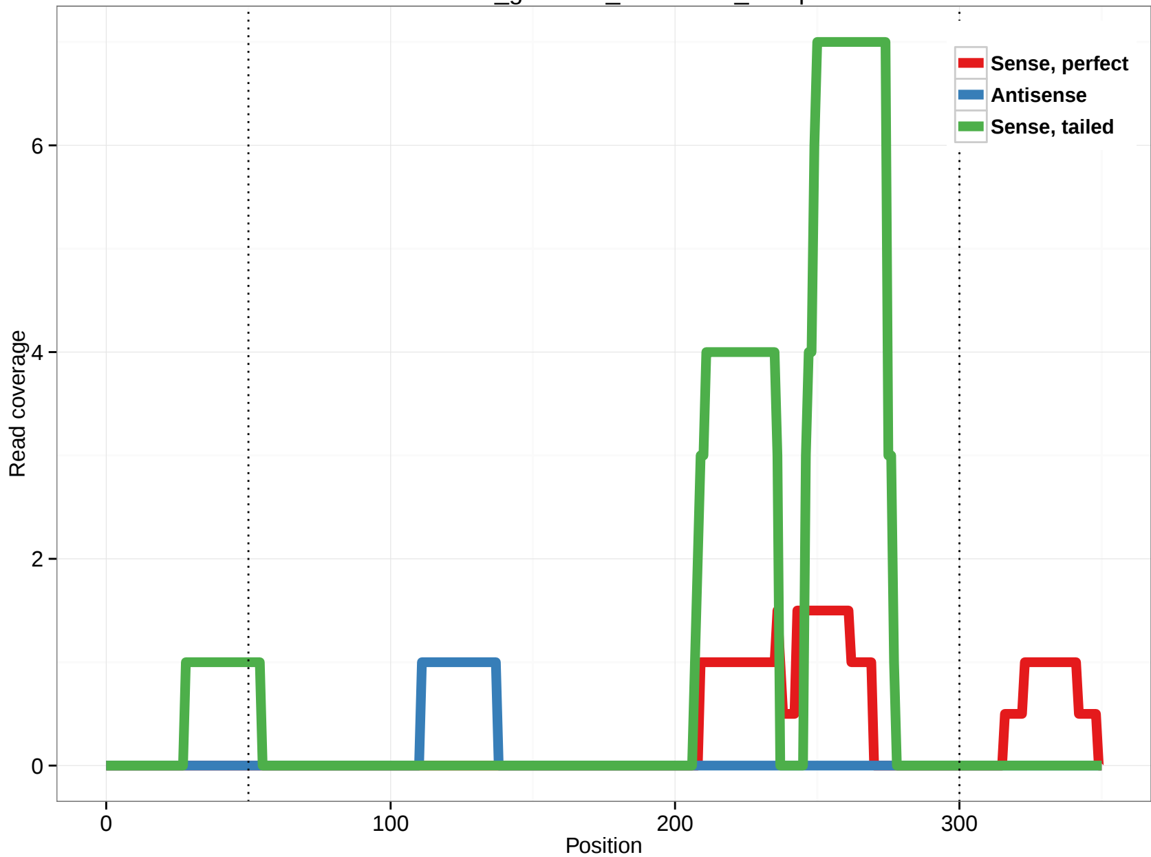
rheMac3_genscan_chr7.1291_11.5p
