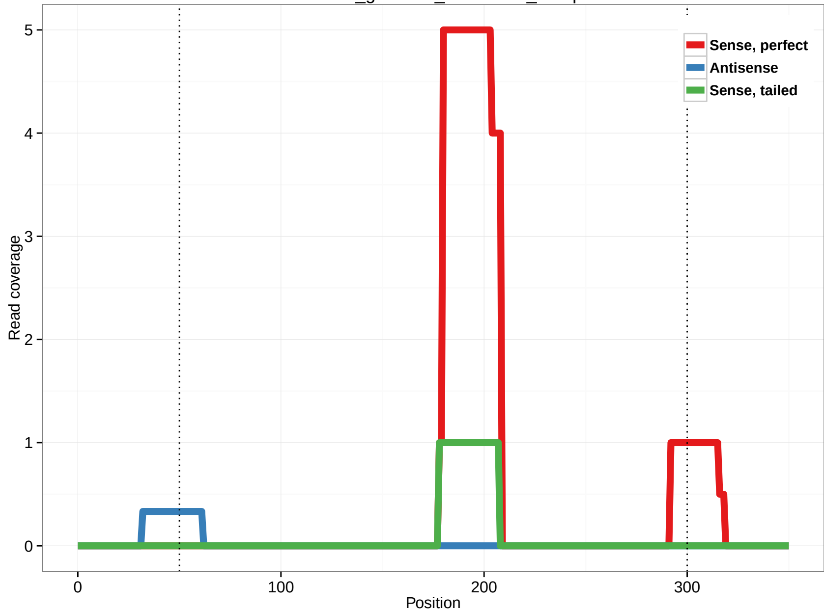
rheMac3_genscan_chr7.1291_10.5p
