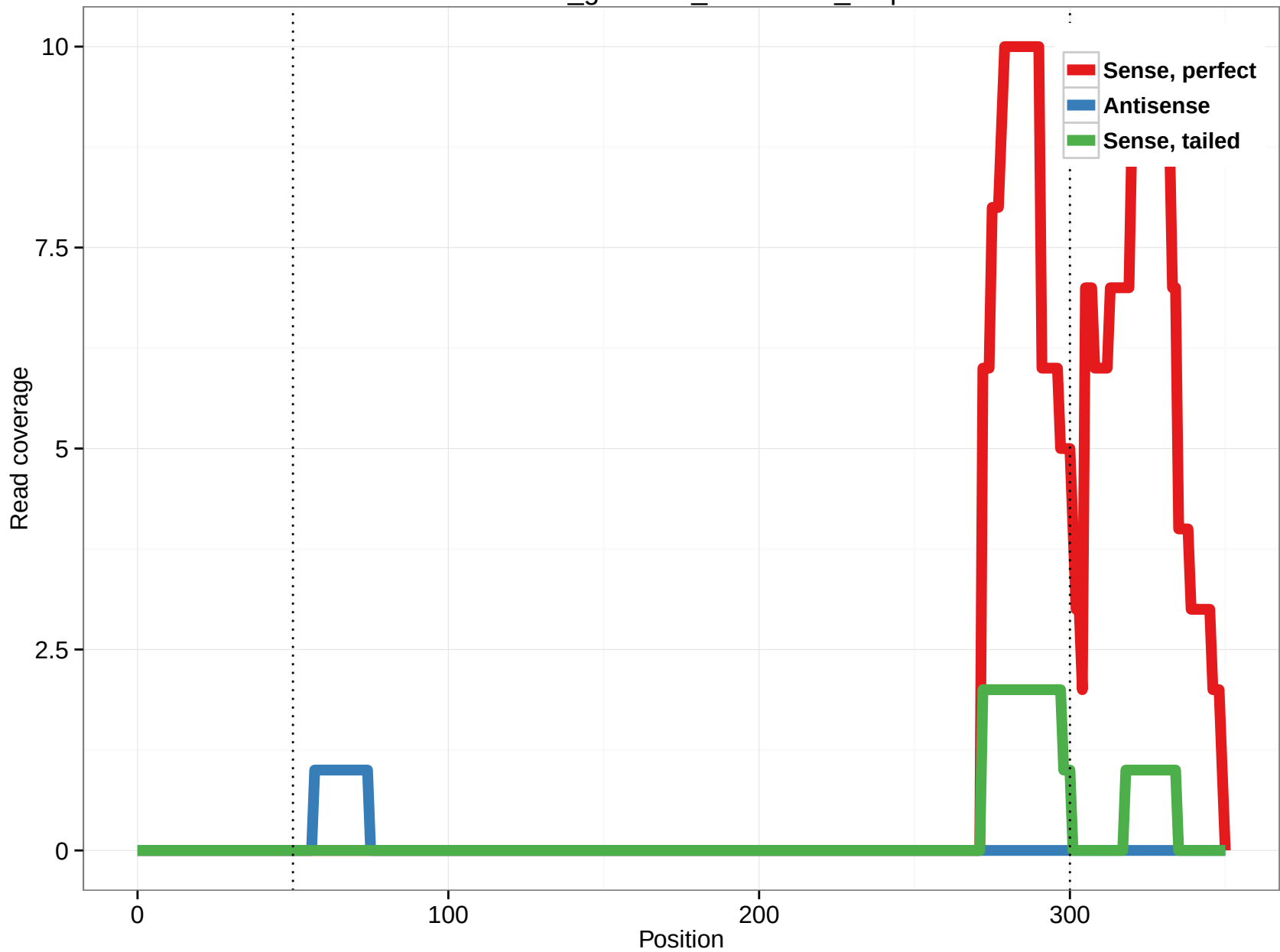
rheMac3_genscan_chr7.1290_2.3p
