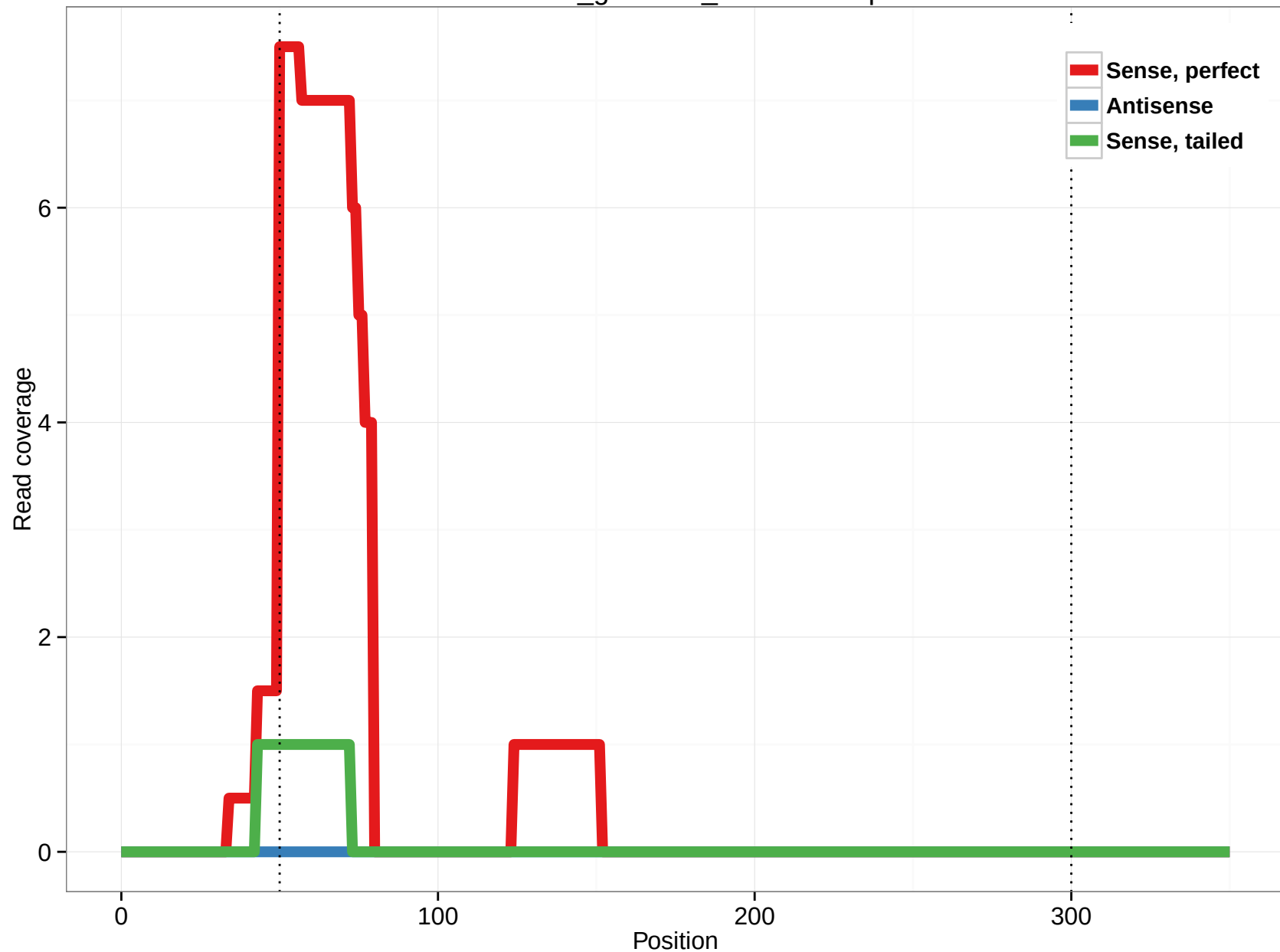
rheMac3_genscan_chr7.1276.5p
